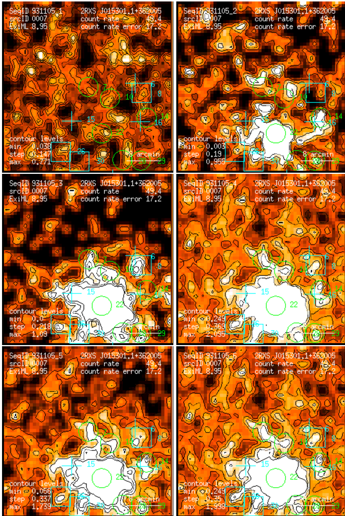
Figure 7: RASS 931105: detection 0007: band rate images, Gaussian filter: (1) PSPC channels 11 – 41, (2) 52 – 90, (3) 91 – 201, (4) 11 – 235, (5) 52 – 201, (6) 11 – 201. Broad band rates in counts/ks. Band rate contour levels in counts/ks/arcmin 2 .
