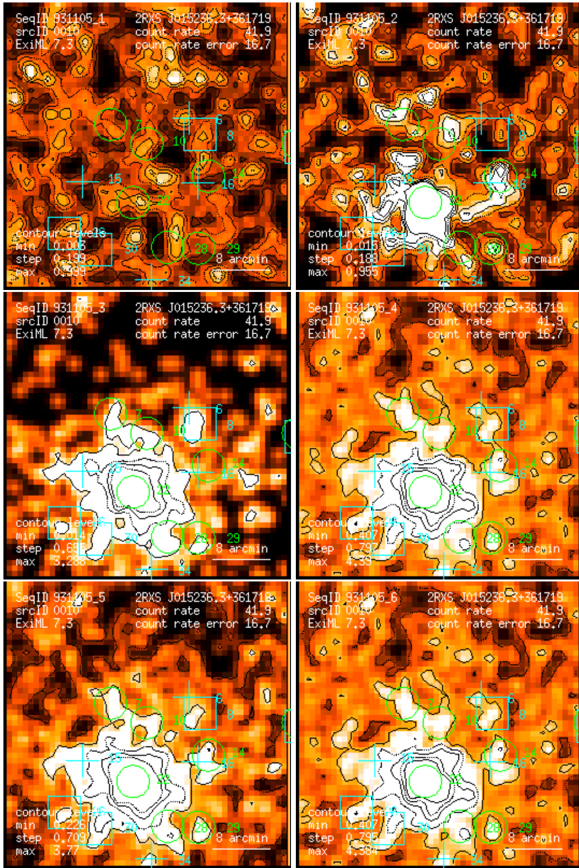
Figure 10: RASS 931105: detection 0010: band rate images, Gaussian filter: (1) PSPC channels 11 – 41, (2) 52 – 90, (3) 91 – 201, (4) 11 – 235, (5) 52 – 201, (6) 11 – 201. Broad band rates in counts/ks. Band rate contour levels in counts/ks/arcmin 2 .
