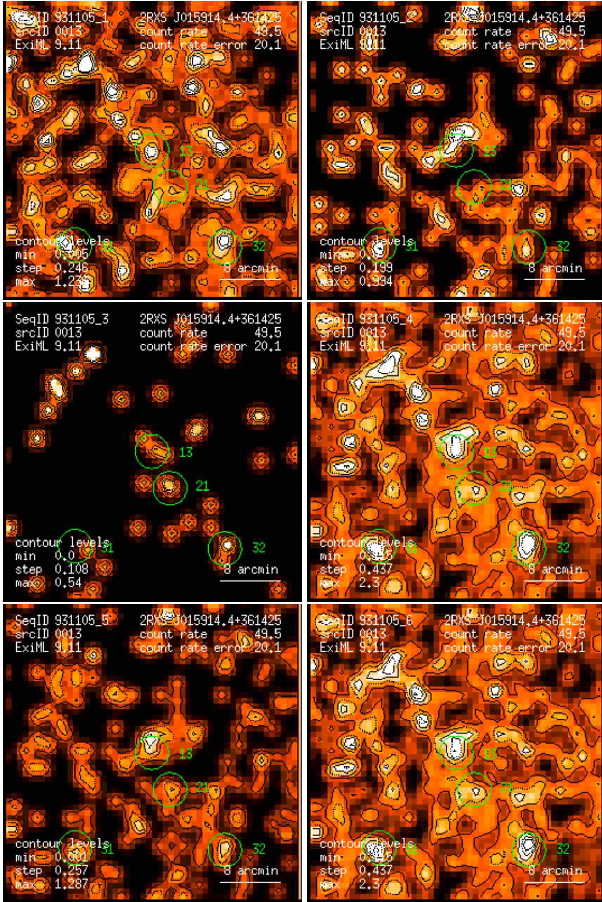
Figure 13: RASS 931105: detection 0013: band rate images, Gaussian filter: (1) PSPC channels 11 – 41, (2) 52 – 90, (3) 91 – 201, (4) 11 – 235, (5) 52 – 201, (6) 11 – 201. Broad band rates in counts/ks. Band rate contour levels in counts/ks/arcmin 2 .
