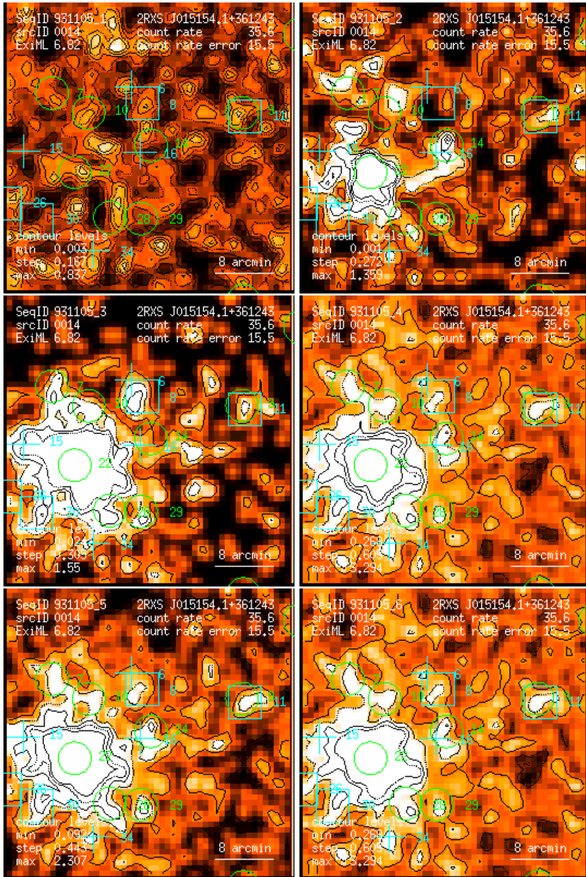
Figure 14: RASS 931105: detection 0014: band rate images, Gaussian filter: (1) PSPC channels 11 – 41, (2) 52 – 90, (3) 91 – 201, (4) 11 – 235, (5) 52 – 201, (6) 11 – 201. Broad band rates in counts/ks. Band rate contour levels in counts/ks/arcmin 2 .
