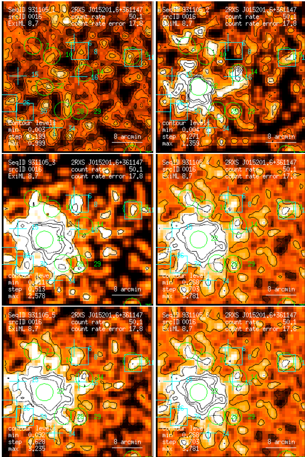
Figure 16: RASS 931105: detection 0016: band rate images, Gaussian filter: (1) PSPC channels 11 – 41, (2) 52 – 90, (3) 91 – 201, (4) 11 – 235, (5) 52 – 201, (6) 11 – 201. Broad band rates in counts/ks. Band rate contour levels in counts/ks/arcmin 2 .
