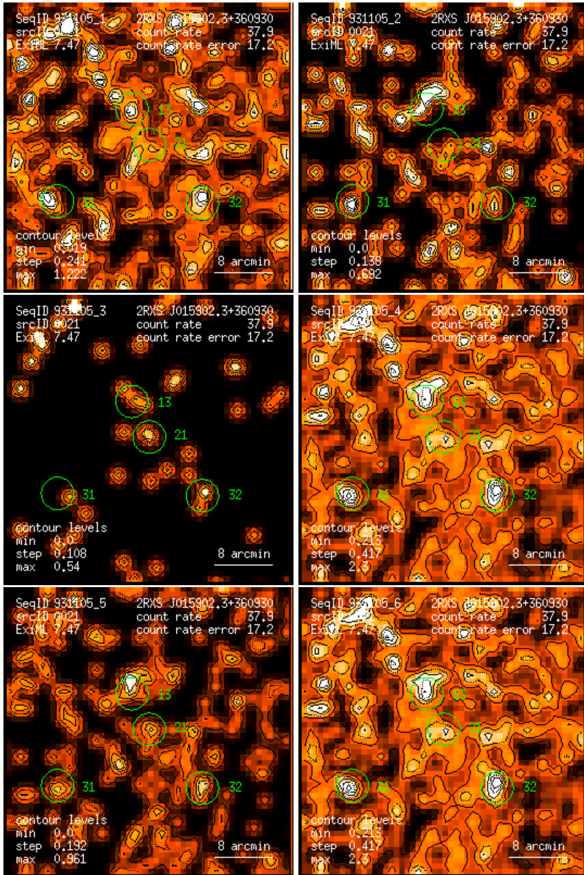
Figure 21: RASS 931105: detection 0021: band rate images, Gaussian filter: (1) PSPC channels 11 – 41, (2) 52 – 90, (3) 91 – 201, (4) 11 – 235, (5) 52 – 201, (6) 11 – 201. Broad band rates in counts/ks. Band rate contour levels in counts/ks/arcmin 2 .
