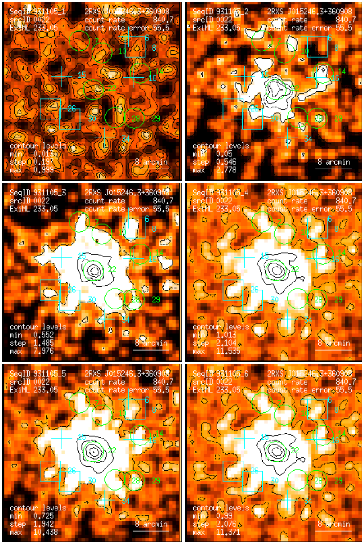
Figure 22: RASS 931105: detection 0022: band rate images, Gaussian filter: (1) PSPC channels 11 – 41, (2) 52 – 90, (3) 91 – 201, (4) 11 – 235, (5) 52 – 201, (6) 11 – 201. Broad band rates in counts/ks. Band rate contour levels in counts/ks/arcmin 2 .
