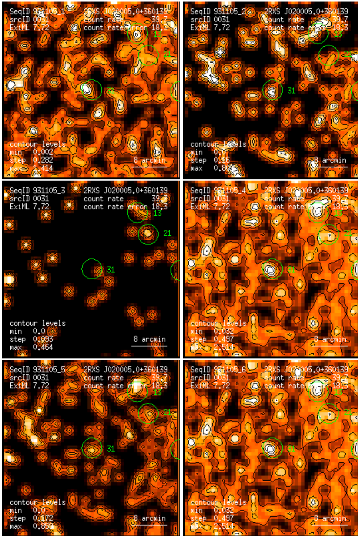
Figure 31: RASS 931105: detection 0031: band rate images, Gaussian filter: (1) PSPC channels 11 – 41, (2) 52 – 90, (3) 91 – 201, (4) 11 – 235, (5) 52 – 201, (6) 11 – 201. Broad band rates in counts/ks. Band rate contour levels in counts/ks/arcmin 2 .
