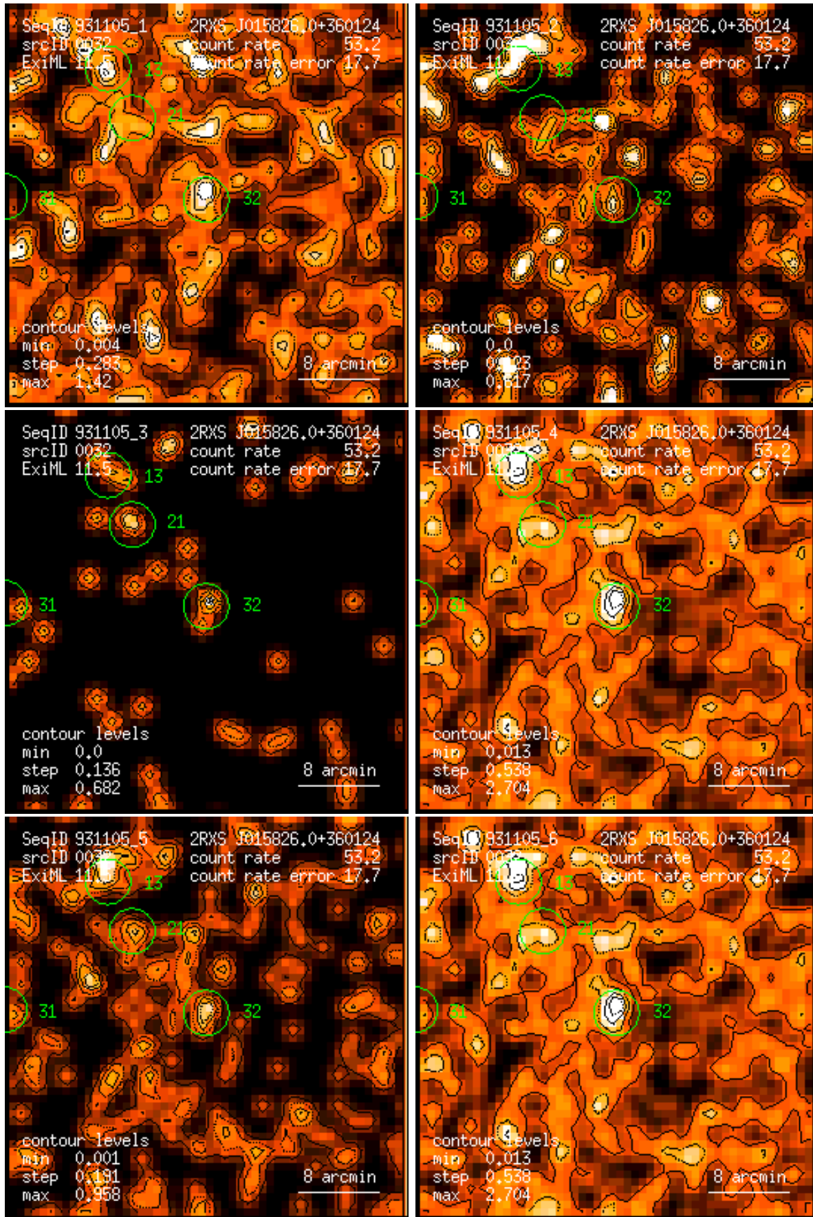
Figure 32: RASS 931105: detection 0032: band rate images, Gaussian filter: (1) PSPC channels 11 – 41, (2) 52 – 90, (3) 91 – 201, (4) 11 – 235, (5) 52 – 201, (6) 11 – 201. Broad band rates in counts/ks. Band rate contour levels in counts/ks/arcmin 2 .
