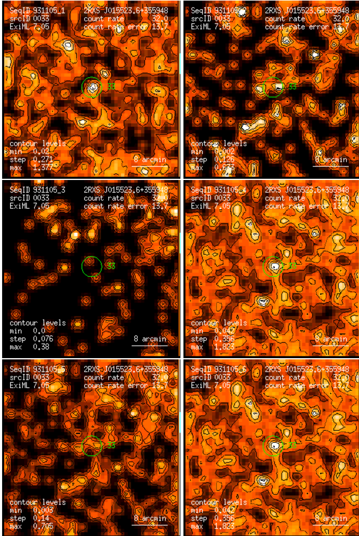
Figure 33: RASS 931105: detection 0033: band rate images, Gaussian filter: (1) PSPC channels 11 – 41, (2) 52 – 90, (3) 91 – 201, (4) 11 – 235, (5) 52 – 201, (6) 11 – 201. Broad band rates in counts/ks. Band rate contour levels in counts/ks/arcmin 2 .
