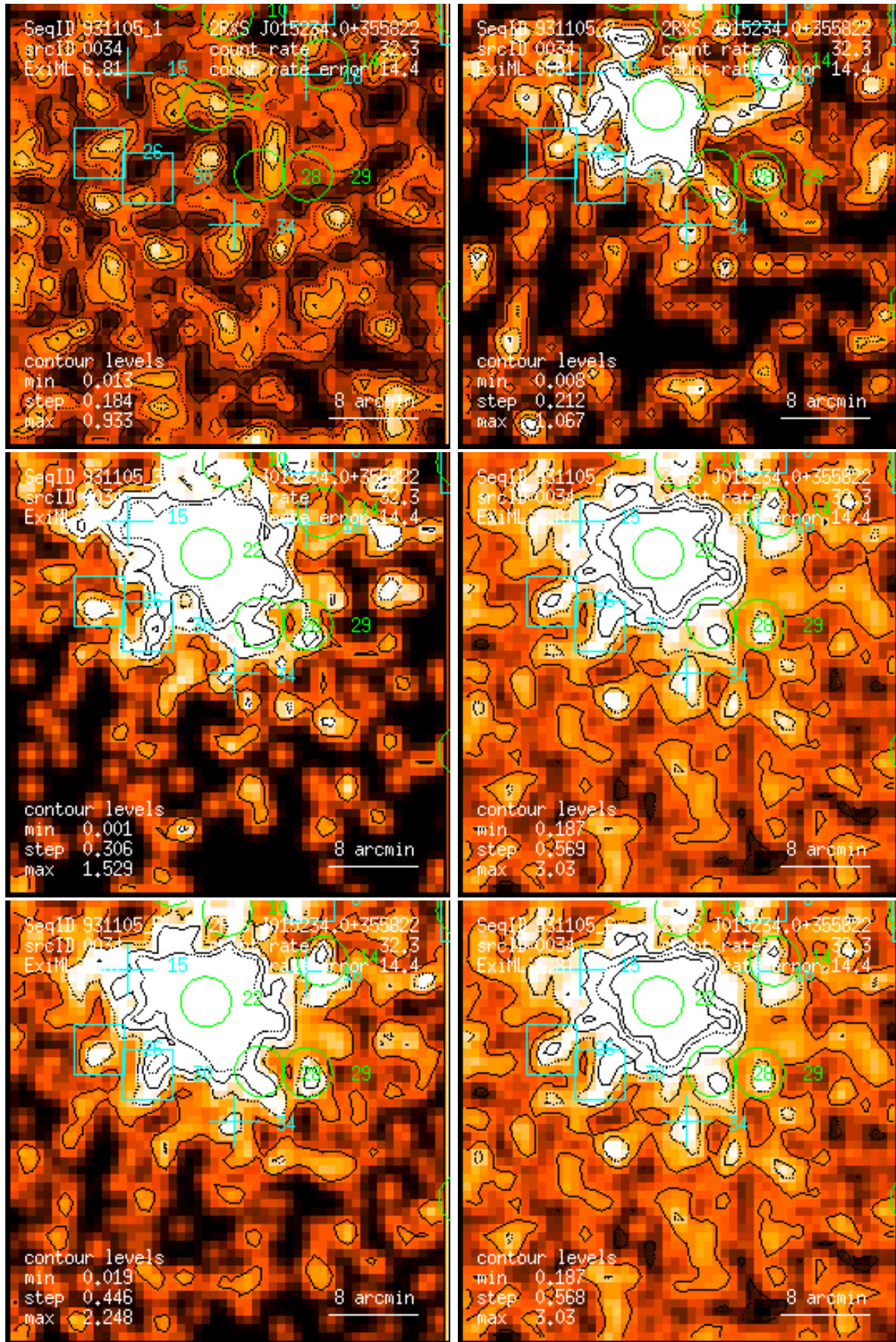
Figure 34: RASS 931105: detection 0034: band rate images, Gaussian filter: (1) PSPC channels 11 – 41, (2) 52 – 90, (3) 91 – 201, (4) 11 – 235, (5) 52 – 201, (6) 11 – 201. Broad band rates in counts/ks. Band rate contour levels in counts/ks/arcmin 2 .
