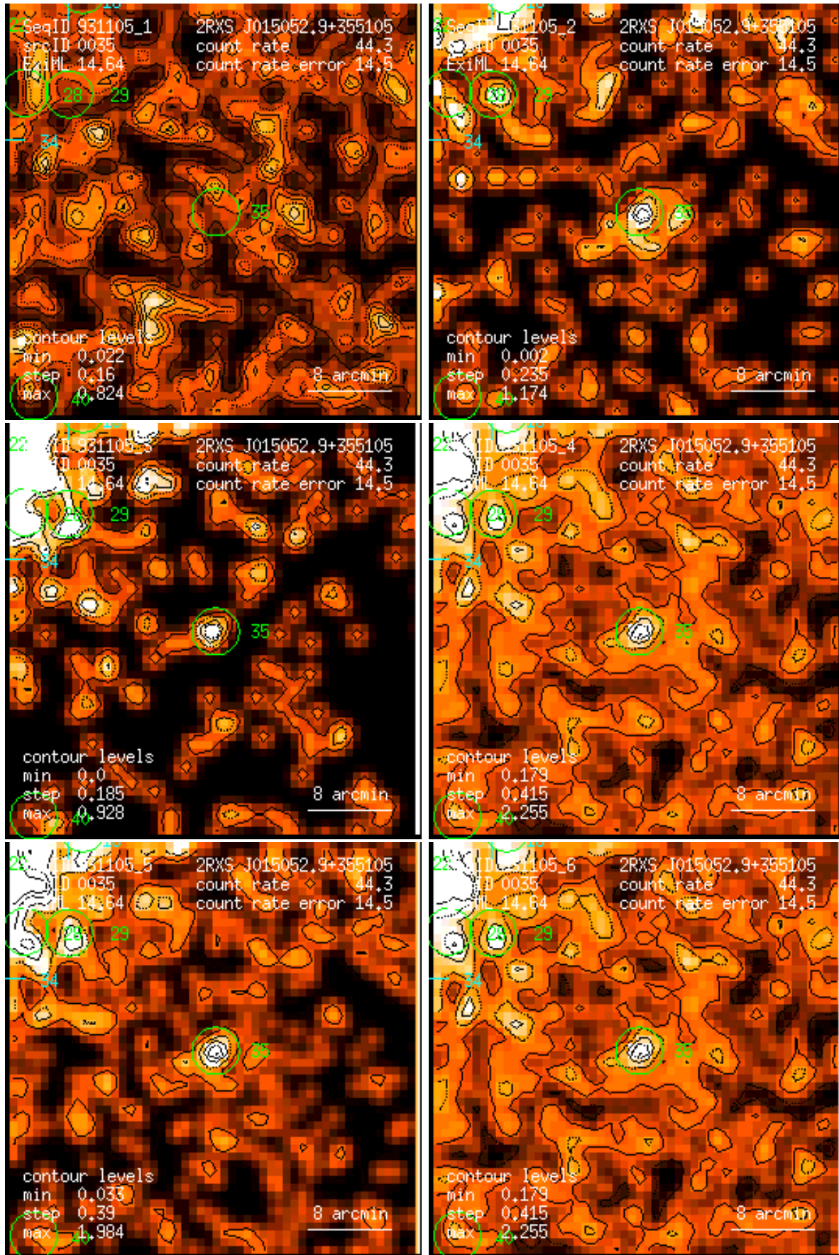
Figure 35: RASS 931105: detection 0035: band rate images, Gaussian filter: (1) PSPC channels 11 – 41, (2) 52 – 90, (3) 91 – 201, (4) 11 – 235, (5) 52 – 201, (6) 11 – 201. Broad band rates in counts/ks. Band rate contour levels in counts/ks/arcmin 2 .
