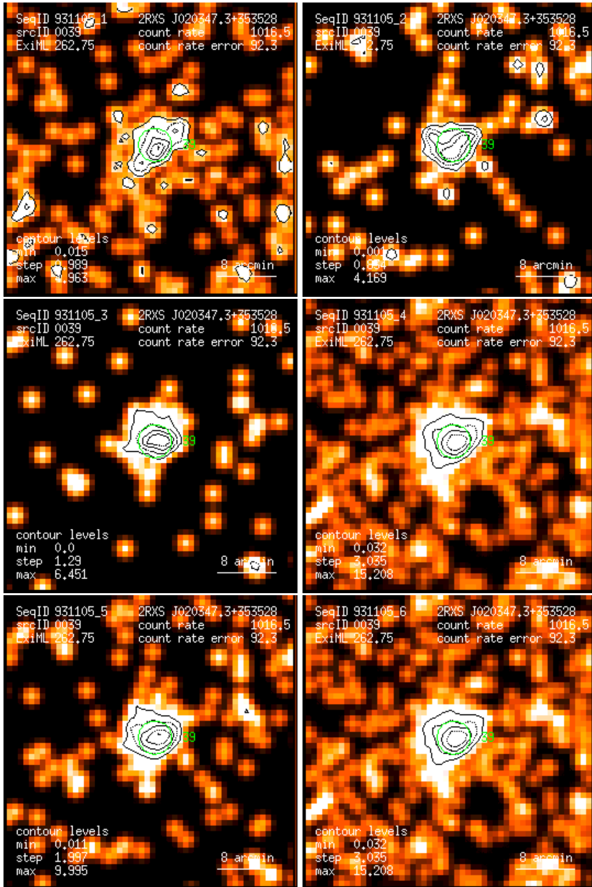
Figure 39: RASS 931105: detection 0039: band rate images, Gaussian filter: (1) PSPC channels 11 – 41, (2) 52 – 90, (3) 91 – 201, (4) 11 – 235, (5) 52 – 201, (6) 11 – 201. Broad band rates in counts/ks. Band rate contour levels in counts/ks/arcmin 2 .
