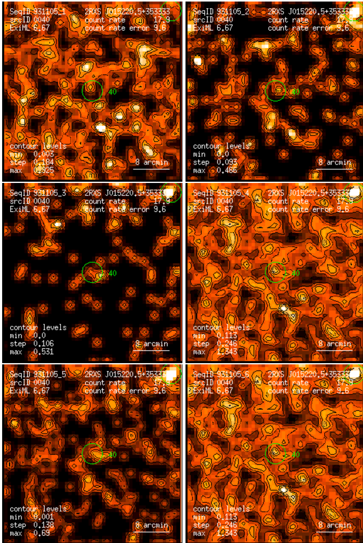
Figure 40: RASS 931105: detection 0040: band rate images, Gaussian filter: (1) PSPC channels 11 – 41, (2) 52 – 90, (3) 91 – 201, (4) 11 – 235, (5) 52 – 201, (6) 11 – 201. Broad band rates in counts/ks. Band rate contour levels in counts/ks/arcmin 2 .
