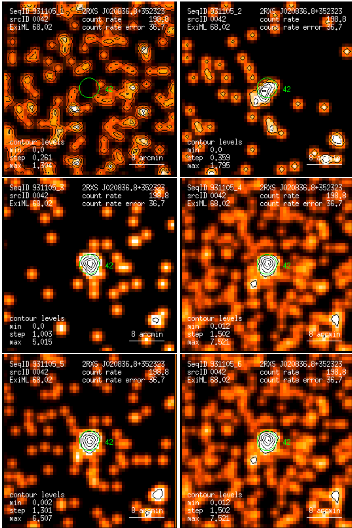
Figure 42: RASS 931105: detection 0042: band rate images, Gaussian filter: (1) PSPC channels 11 – 41, (2) 52 – 90, (3) 91 – 201, (4) 11 – 235, (5) 52 – 201, (6) 11 – 201. Broad band rates in counts/ks. Band rate contour levels in counts/ks/arcmin 2 .
