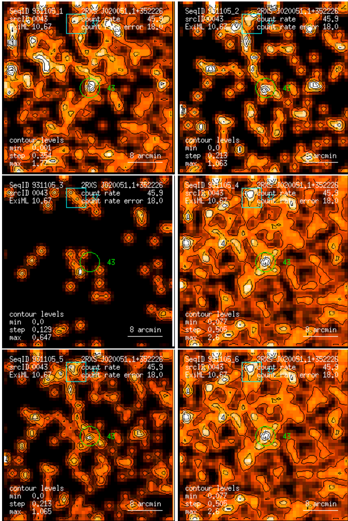
Figure 43: RASS 931105: detection 0043: band rate images, Gaussian filter: (1) PSPC channels 11 – 41, (2) 52 – 90, (3) 91 – 201, (4) 11 – 235, (5) 52 – 201, (6) 11 – 201. Broad band rates in counts/ks. Band rate contour levels in counts/ks/arcmin 2 .
