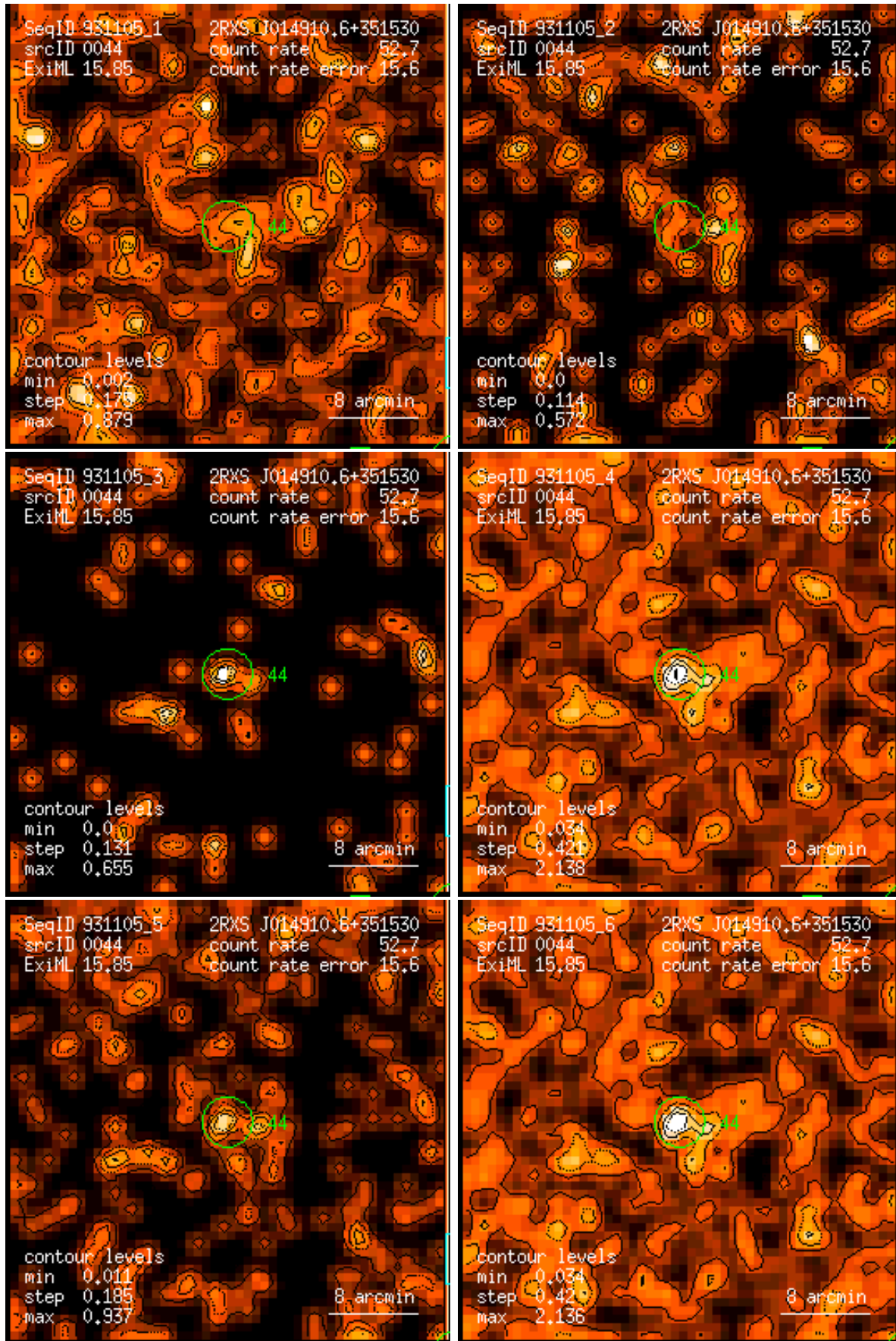
Figure 44: RASS 931105: detection 0044: band rate images, Gaussian filter: (1) PSPC channels 11 – 41, (2) 52 – 90, (3) 91 – 201, (4) 11 – 235, (5) 52 – 201, (6) 11 – 201. Broad band rates in counts/ks. Band rate contour levels in counts/ks/arcmin 2 .
