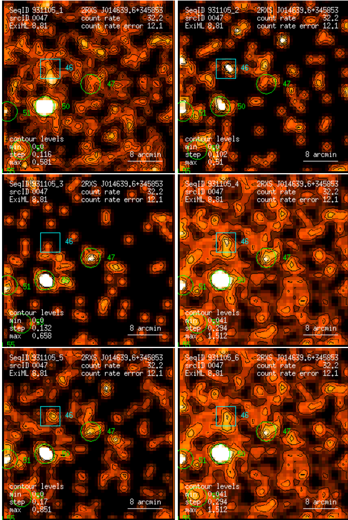
Figure 47: RASS 931105: detection 0047: band rate images, Gaussian filter: (1) PSPC channels 11 – 41, (2) 52 – 90, (3) 91 – 201, (4) 11 – 235, (5) 52 – 201, (6) 11 – 201. Broad band rates in counts/ks. Band rate contour levels in counts/ks/arcmin 2 .
