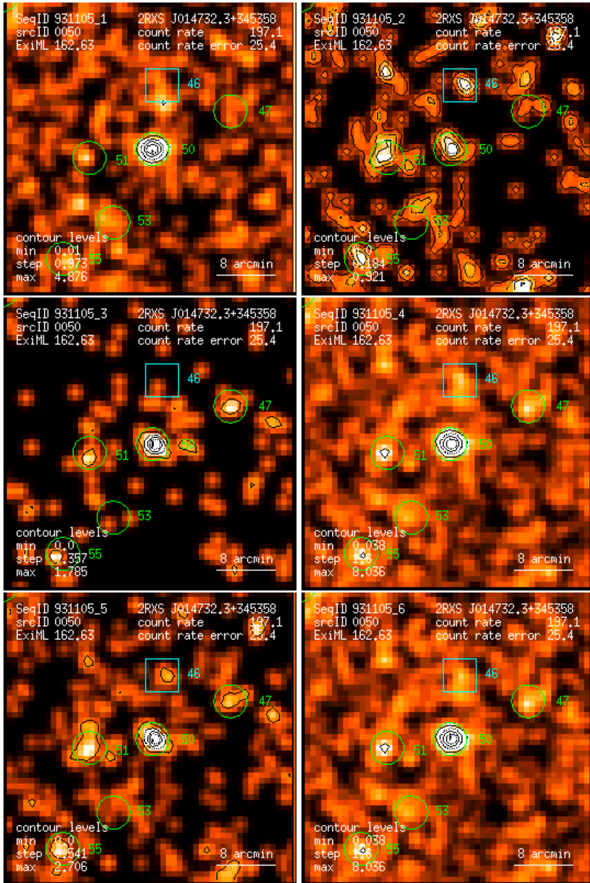
Figure 50: RASS 931105: detection 0050: band rate images, Gaussian filter: (1) PSPC channels 11 – 41, (2) 52 – 90, (3) 91 – 201, (4) 11 – 235, (5) 52 – 201, (6) 11 – 201. Broad band rates in counts/ks. Band rate contour levels in counts/ks/arcmin 2 .
