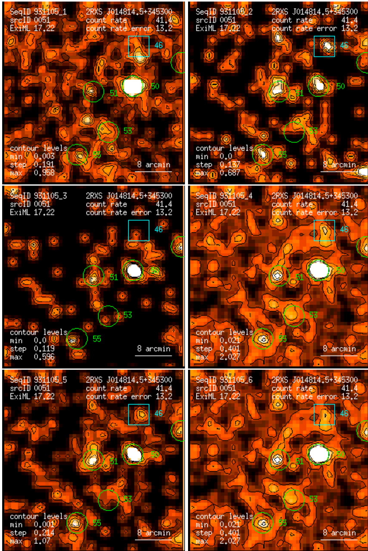
Figure 51: RASS 931105: detection 0051: band rate images, Gaussian filter: (1) PSPC channels 11 – 41, (2) 52 – 90, (3) 91 – 201, (4) 11 – 235, (5) 52 – 201, (6) 11 – 201. Broad band rates in counts/ks. Band rate contour levels in counts/ks/arcmin 2 .
