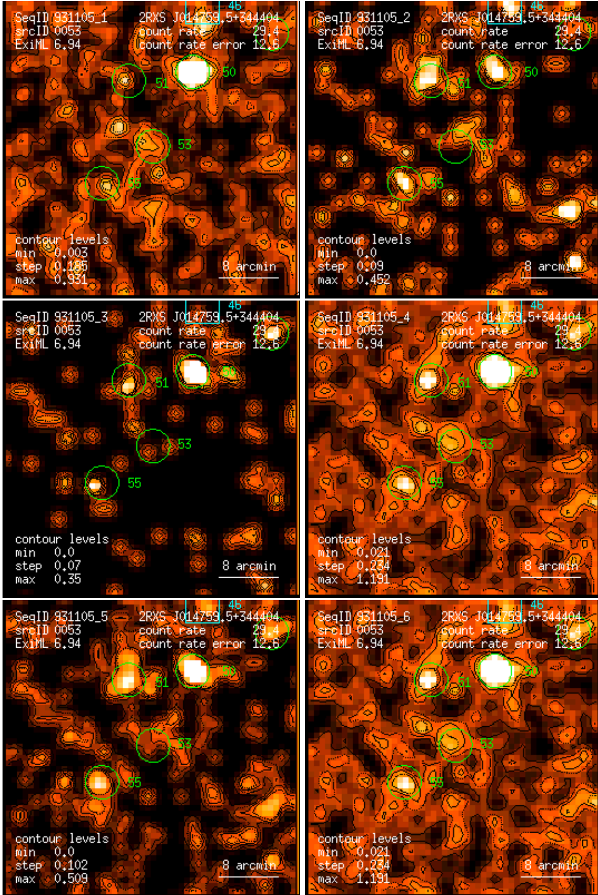
Figure 53: RASS 931105: detection 0053: band rate images, Gaussian filter: (1) PSPC channels 11 – 41, (2) 52 – 90, (3) 91 – 201, (4) 11 – 235, (5) 52 – 201, (6) 11 – 201. Broad band rates in counts/ks. Band rate contour levels in counts/ks/arcmin 2 .
