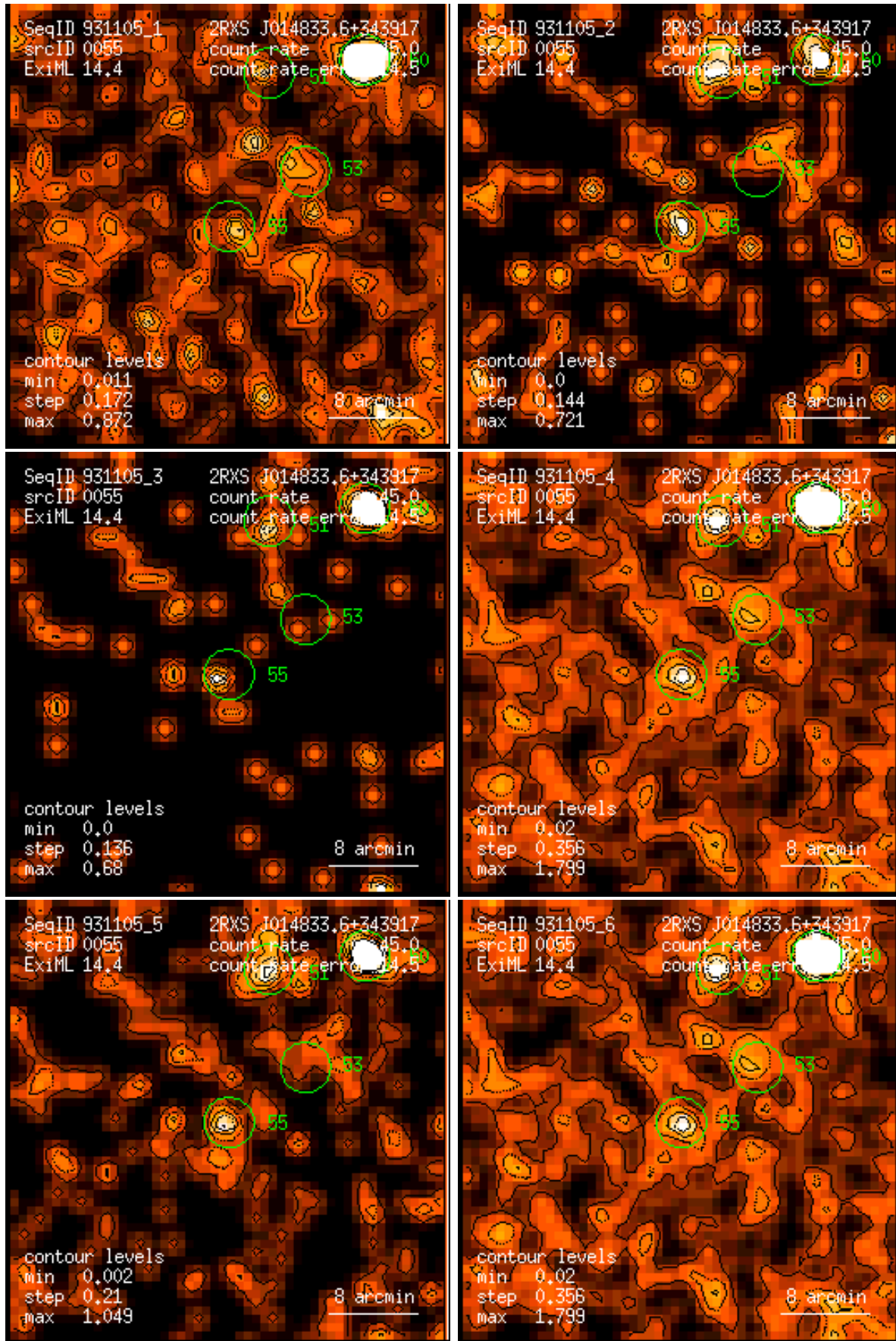
Figure 55: RASS 931105: detection 0055: band rate images, Gaussian filter: (1) PSPC channels 11 – 41, (2) 52 – 90, (3) 91 – 201, (4) 11 – 235, (5) 52 – 201, (6) 11 – 201. Broad band rates in counts/ks. Band rate contour levels in counts/ks/arcmin 2 .
