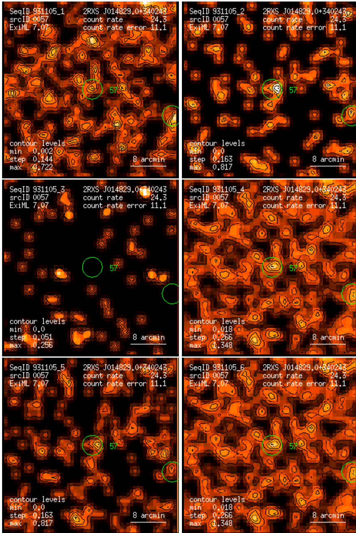
Figure 57: RASS 931105: detection 0057: band rate images, Gaussian filter: (1) PSPC channels 11 – 41, (2) 52 – 90, (3) 91 – 201, (4) 11 – 235, (5) 52 – 201, (6) 11 – 201. Broad band rates in counts/ks. Band rate contour levels in counts/ks/arcmin 2 .
