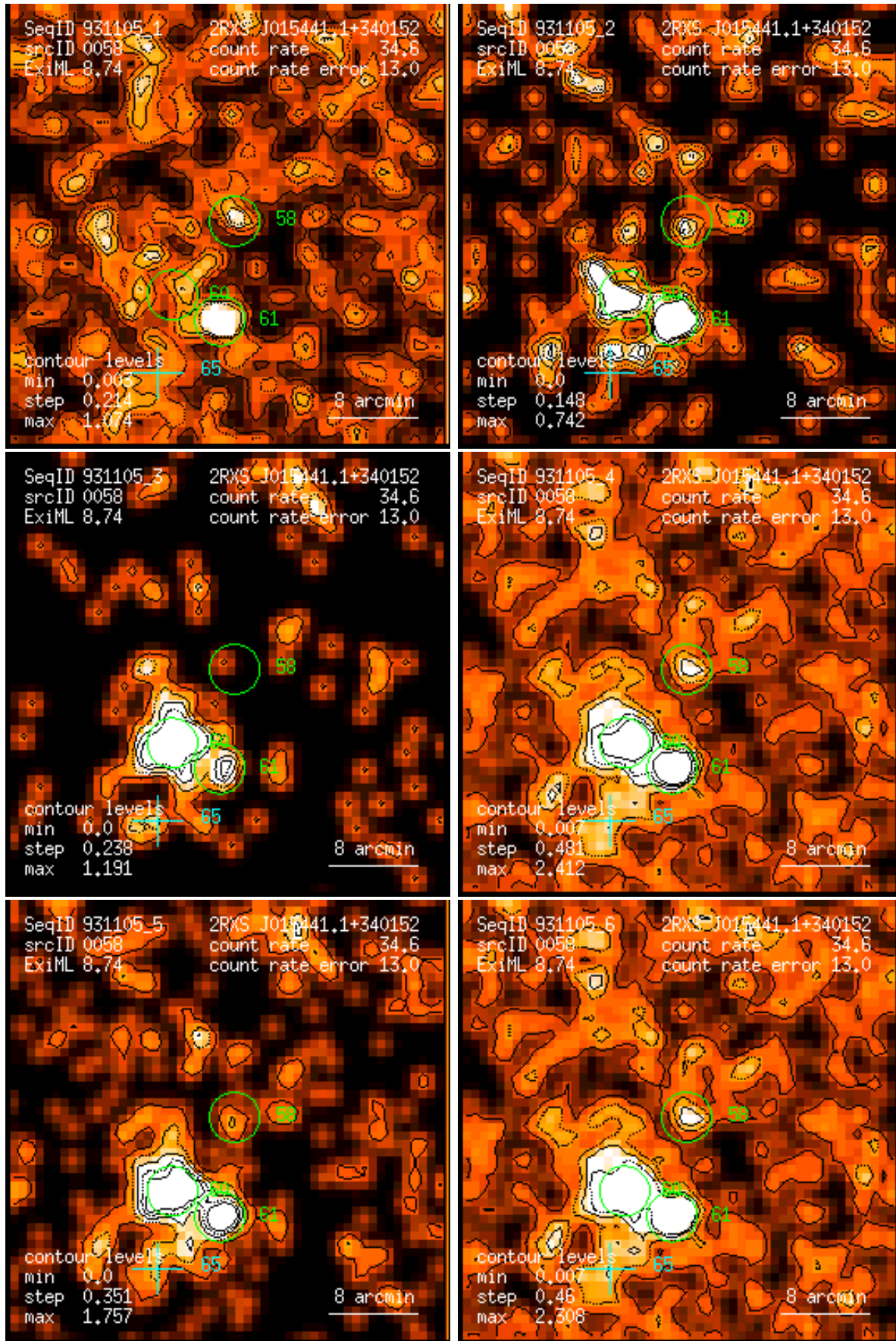
Figure 58: RASS 931105: detection 0058: band rate images, Gaussian filter: (1) PSPC channels 11 – 41, (2) 52 – 90, (3) 91 – 201, (4) 11 – 235, (5) 52 – 201, (6) 11 – 201. Broad band rates in counts/ks. Band rate contour levels in counts/ks/arcmin 2 .
