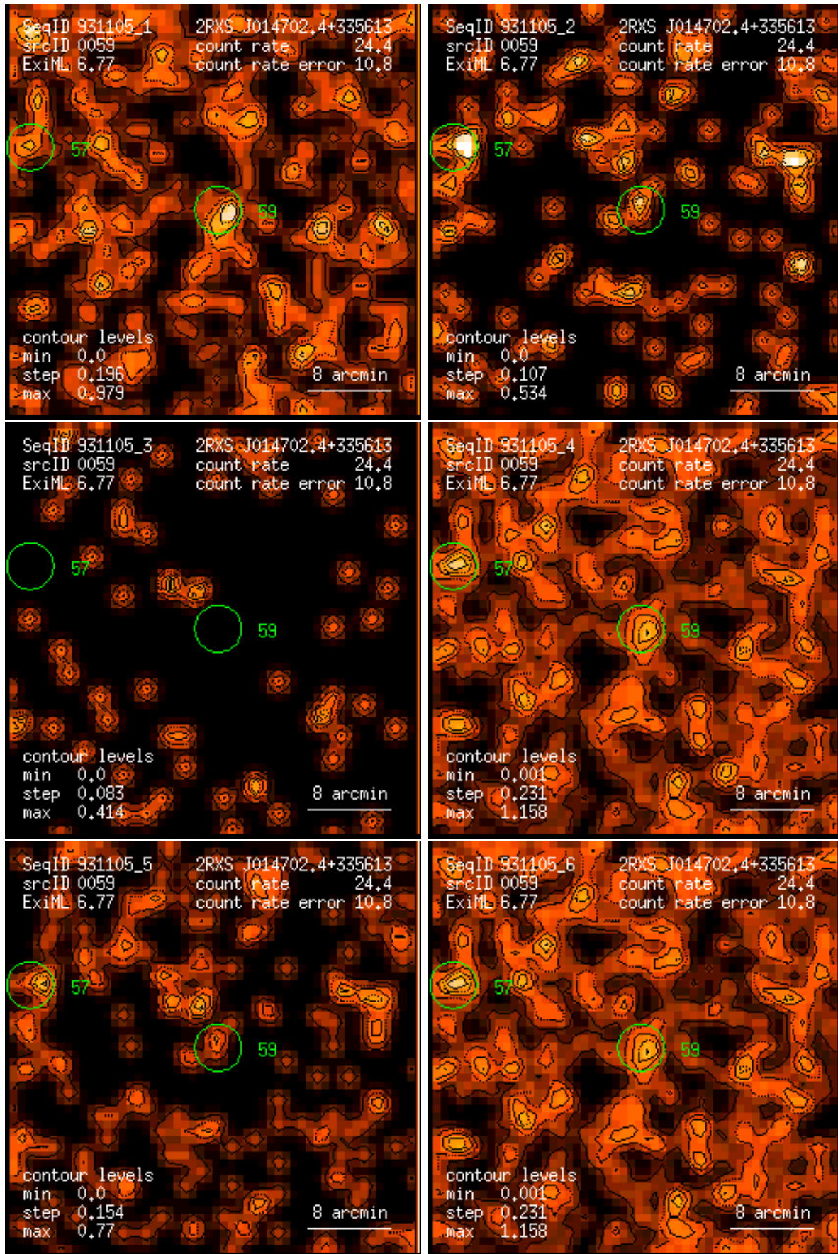
Figure 59: RASS 931105: detection 0059: band rate images, Gaussian filter: (1) PSPC channels 11 – 41, (2) 52 – 90, (3) 91 – 201, (4) 11 – 235, (5) 52 – 201, (6) 11 – 201. Broad band rates in counts/ks. Band rate contour levels in counts/ks/arcmin 2 .
