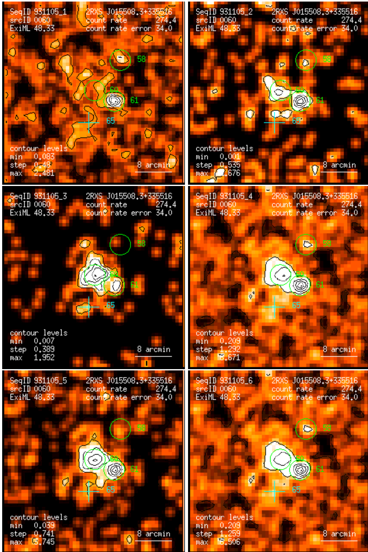
Figure 60: RASS 931105: detection 0060: band rate images, Gaussian filter: (1) PSPC channels 11 – 41, (2) 52 – 90, (3) 91 – 201, (4) 11 – 235, (5) 52 – 201, (6) 11 – 201. Broad band rates in counts/ks. Band rate contour levels in counts/ks/arcmin 2 .
