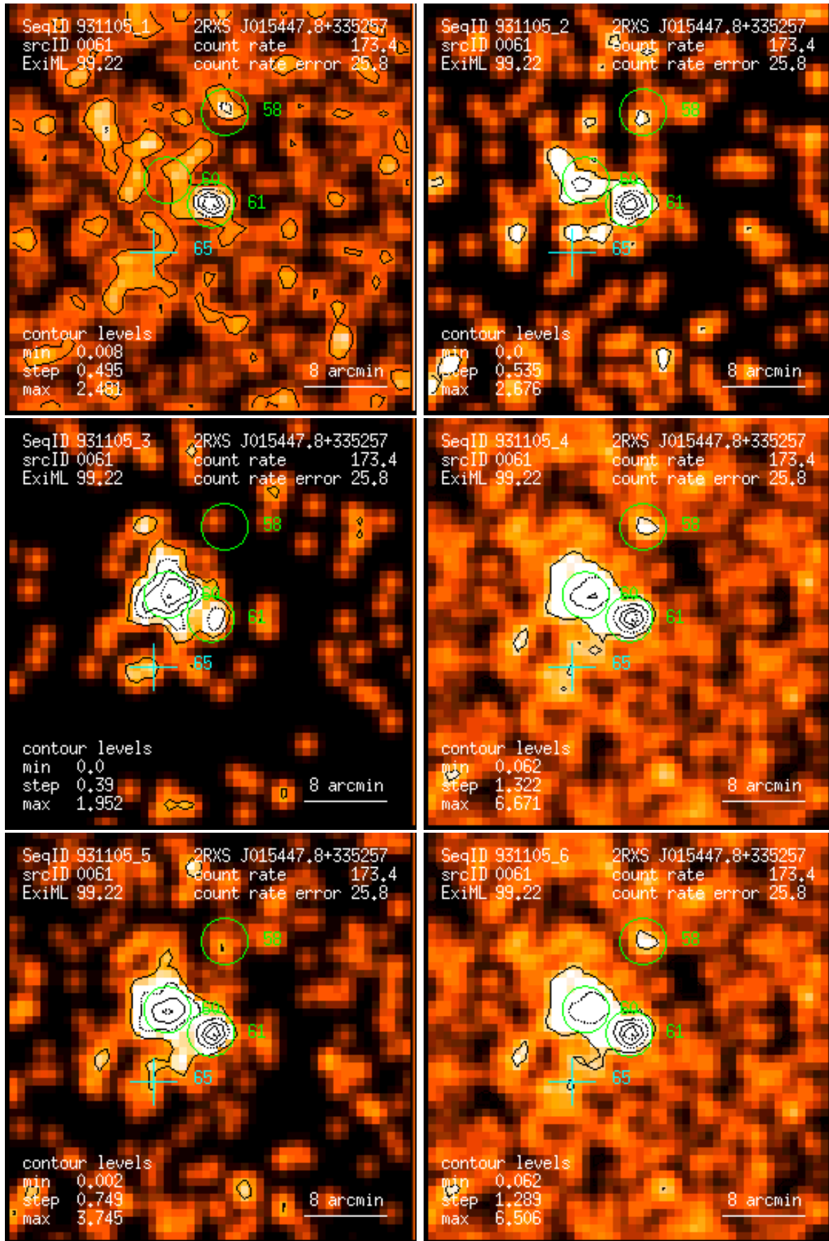
Figure 61: RASS 931105: detection 0061: band rate images, Gaussian filter: (1) PSPC channels 11 – 41, (2) 52 – 90, (3) 91 – 201, (4) 11 – 235, (5) 52 – 201, (6) 11 – 201. Broad band rates in counts/ks. Band rate contour levels in counts/ks/arcmin 2 .
