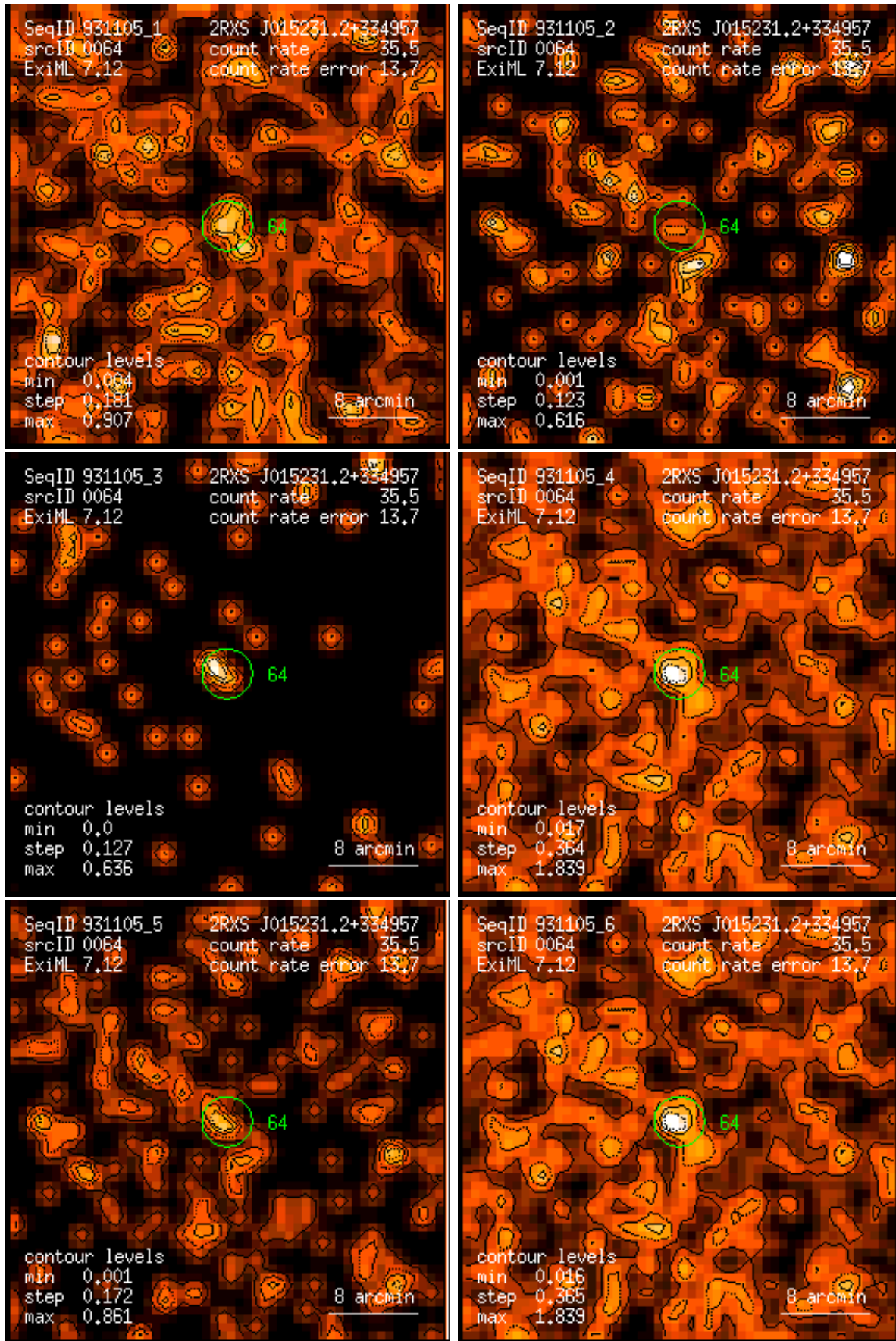
Figure 64: RASS 931105: detection 0064: band rate images, Gaussian filter: (1) PSPC channels 11 – 41, (2) 52 – 90, (3) 91 – 201, (4) 11 – 235, (5) 52 – 201, (6) 11 – 201. Broad band rates in counts/ks. Band rate contour levels in counts/ks/arcmin 2 .
