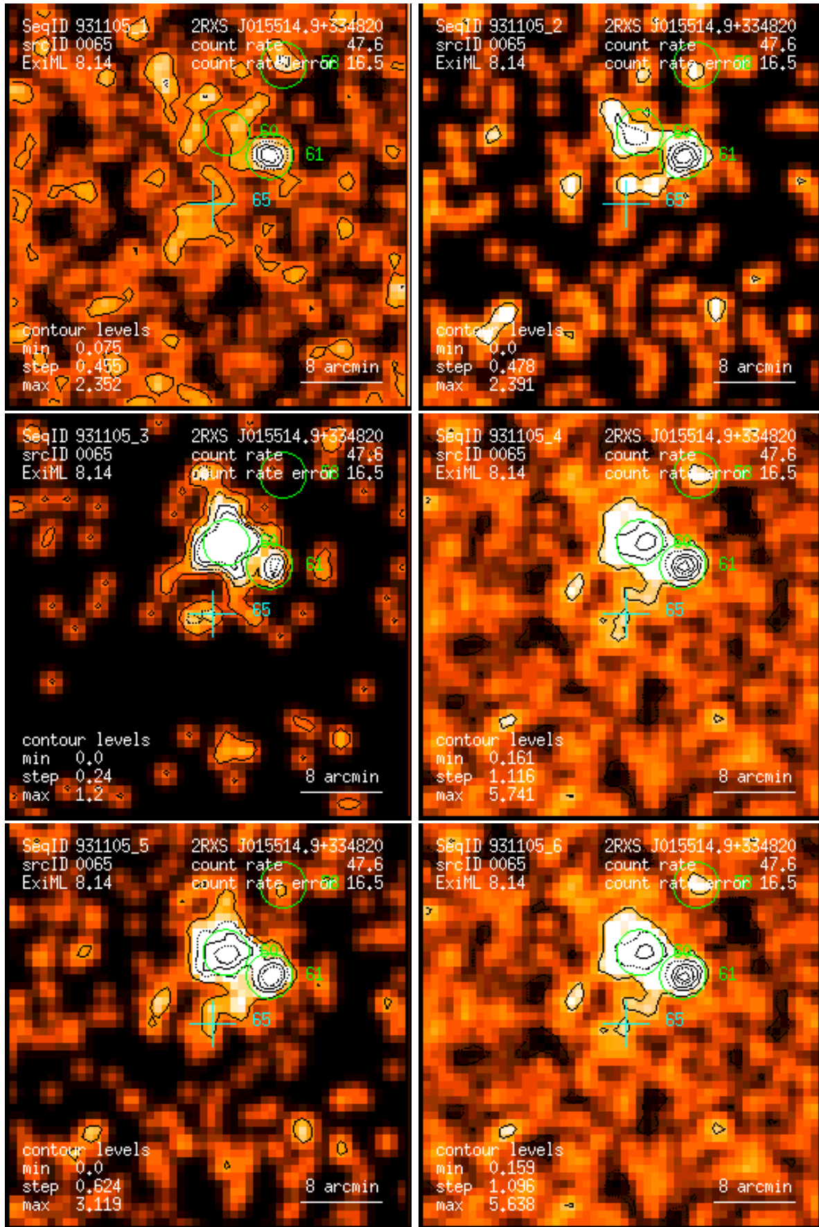
Figure 65: RASS 931105: detection 0065: band rate images, Gaussian filter: (1) PSPC channels 11 – 41, (2) 52 – 90, (3) 91 – 201, (4) 11 – 235, (5) 52 – 201, (6) 11 – 201. Broad band rates in counts/ks. Band rate contour levels in counts/ks/arcmin 2 .
