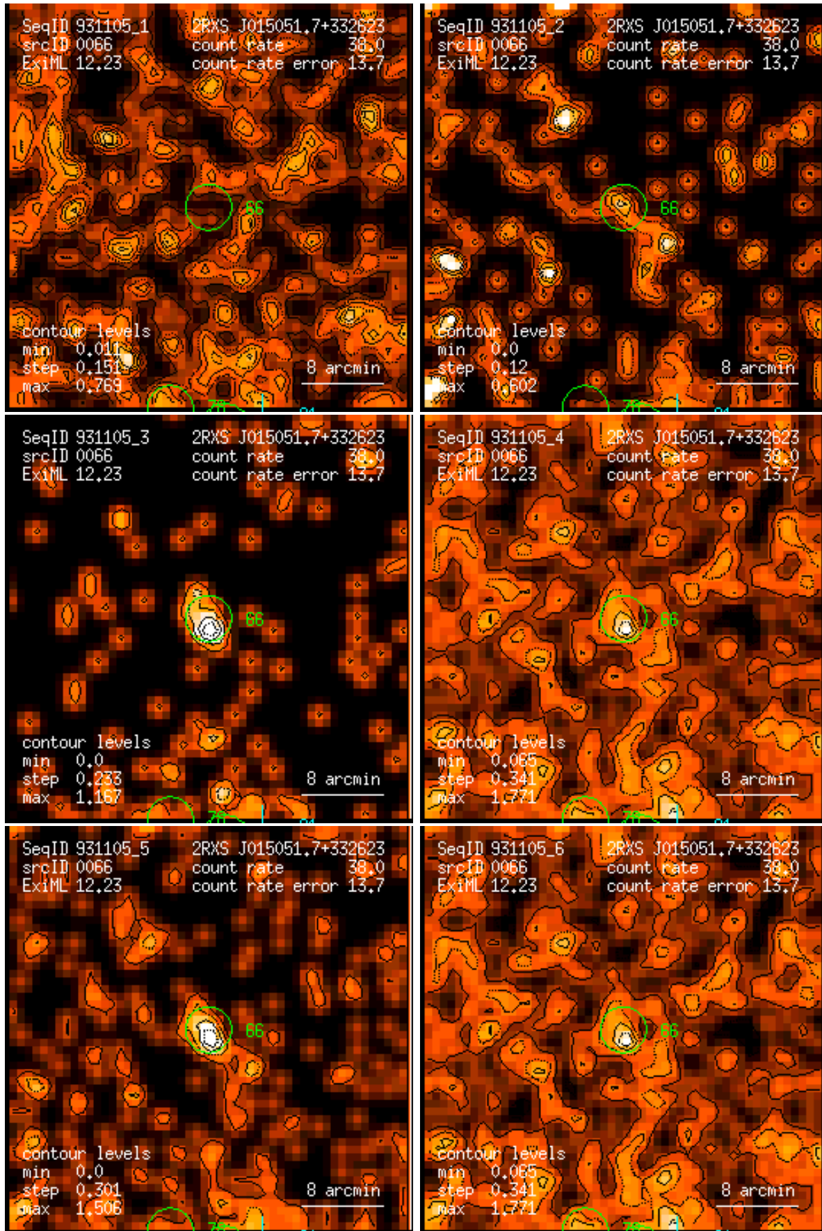
Figure 66: RASS 931105: detection 0066: band rate images, Gaussian filter: (1) PSPC channels 11 – 41, (2) 52 – 90, (3) 91 – 201, (4) 11 – 235, (5) 52 – 201, (6) 11 – 201. Broad band rates in counts/ks. Band rate contour levels in counts/ks/arcmin 2 .
