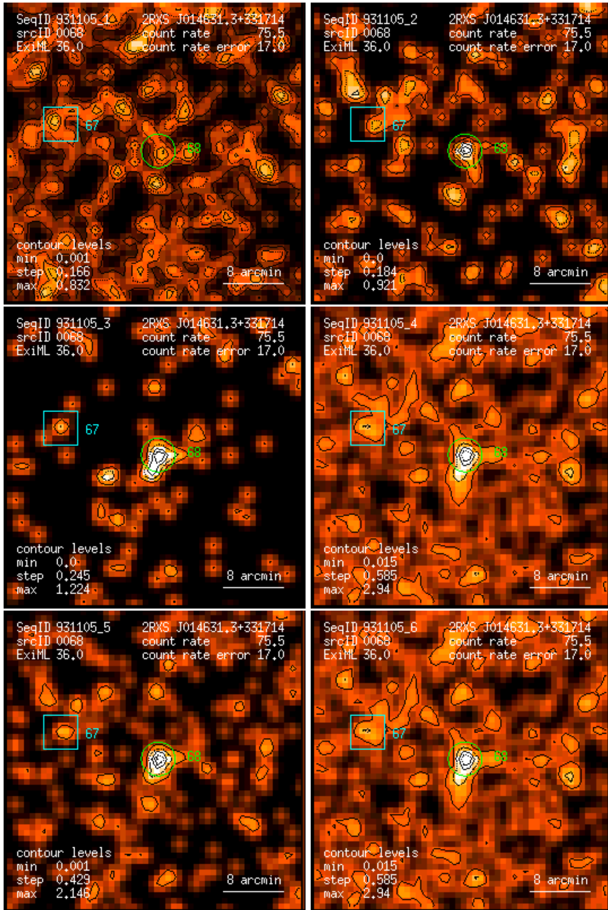
Figure 68: RASS 931105: detection 0068: band rate images, Gaussian filter: (1) PSPC channels 11 – 41, (2) 52 – 90, (3) 91 – 201, (4) 11 – 235, (5) 52 – 201, (6) 11 – 201. Broad band rates in counts/ks. Band rate contour levels in counts/ks/arcmin 2 .
