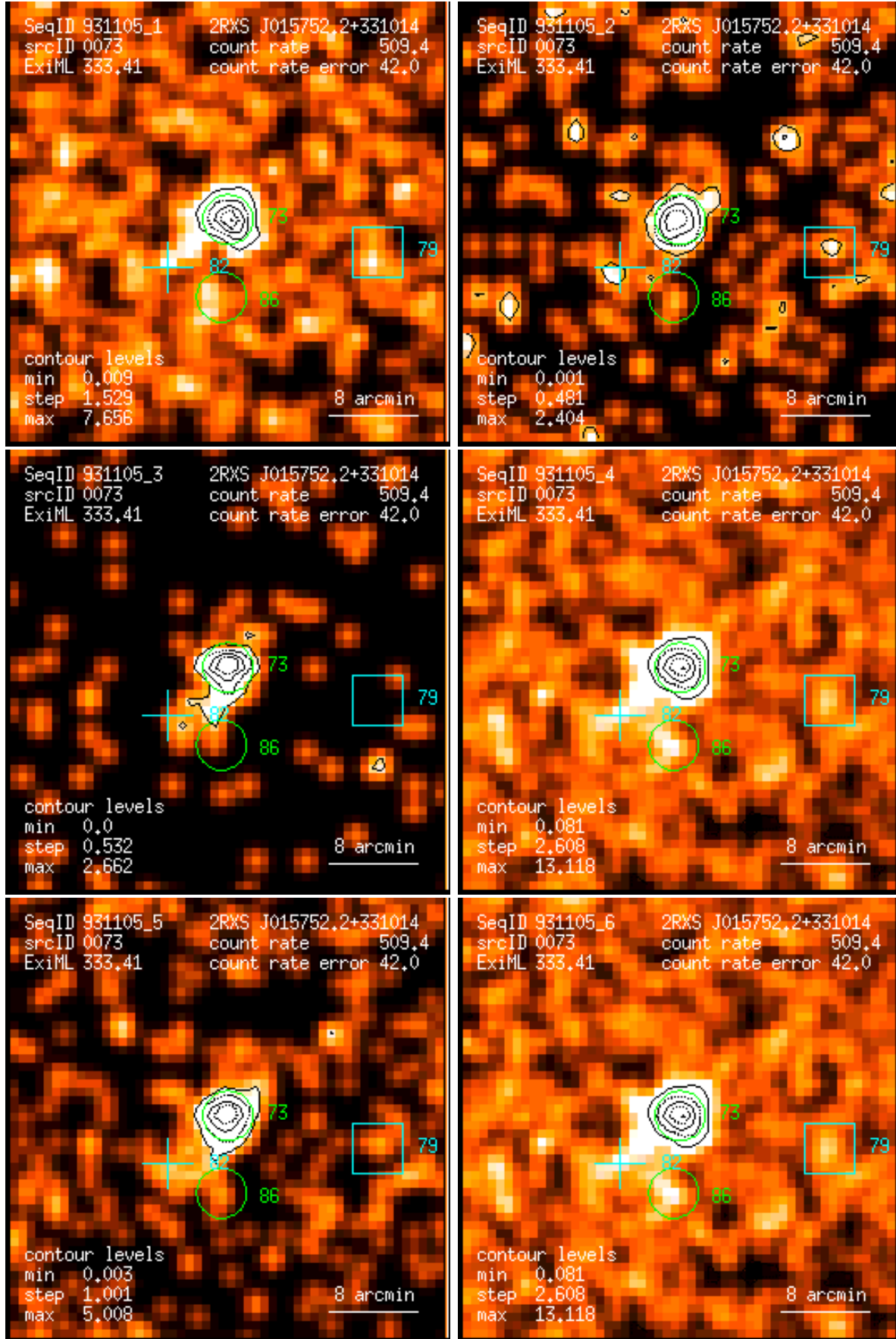
Figure 73: RASS 931105: detection 0073: band rate images, Gaussian filter: (1) PSPC channels 11 – 41, (2) 52 – 90, (3) 91 – 201, (4) 11 – 235, (5) 52 – 201, (6) 11 – 201. Broad band rates in counts/ks. Band rate contour levels in counts/ks/arcmin 2 .
