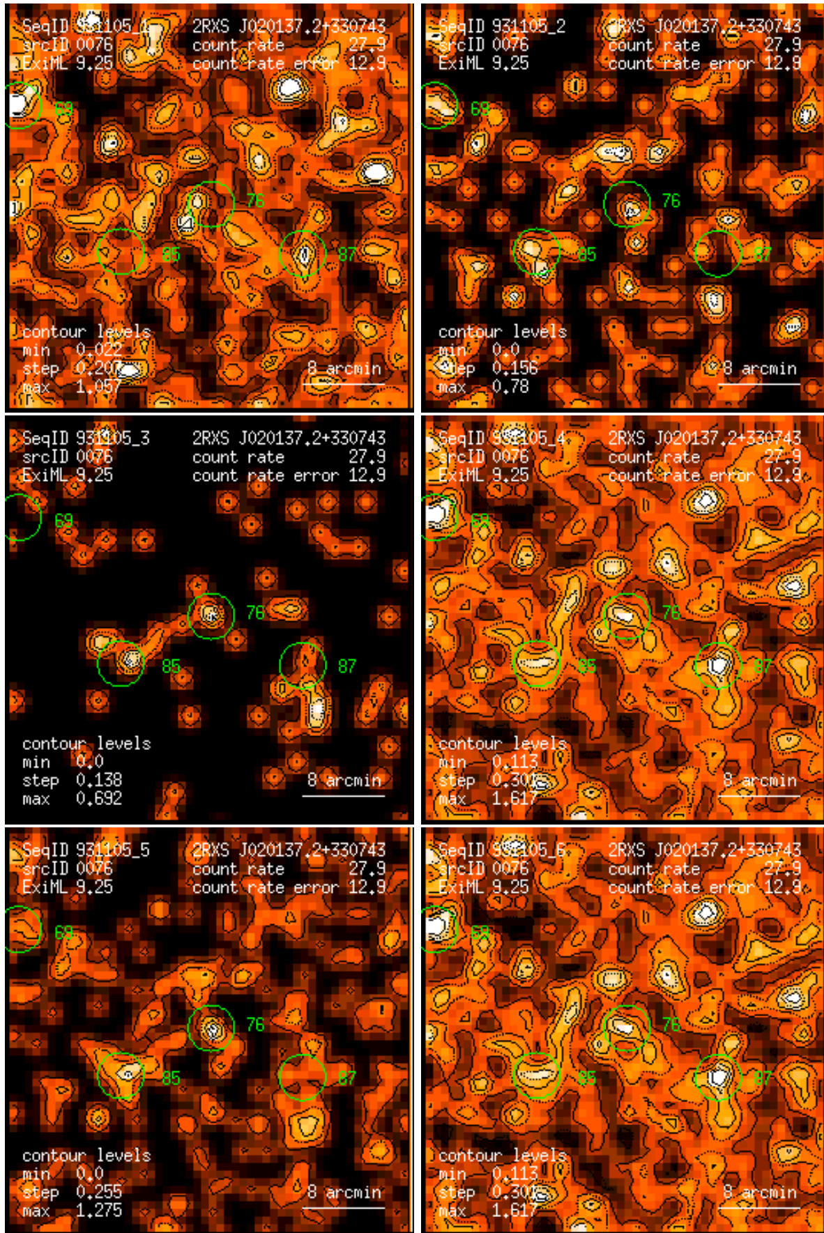
Figure 76: RASS 931105: detection 0076: band rate images, Gaussian filter: (1) PSPC channels 11 – 41, (2) 52 – 90, (3) 91 – 201, (4) 11 – 235, (5) 52 – 201, (6) 11 – 201. Broad band rates in counts/ks. Band rate contour levels in counts/ks/arcmin 2 .
