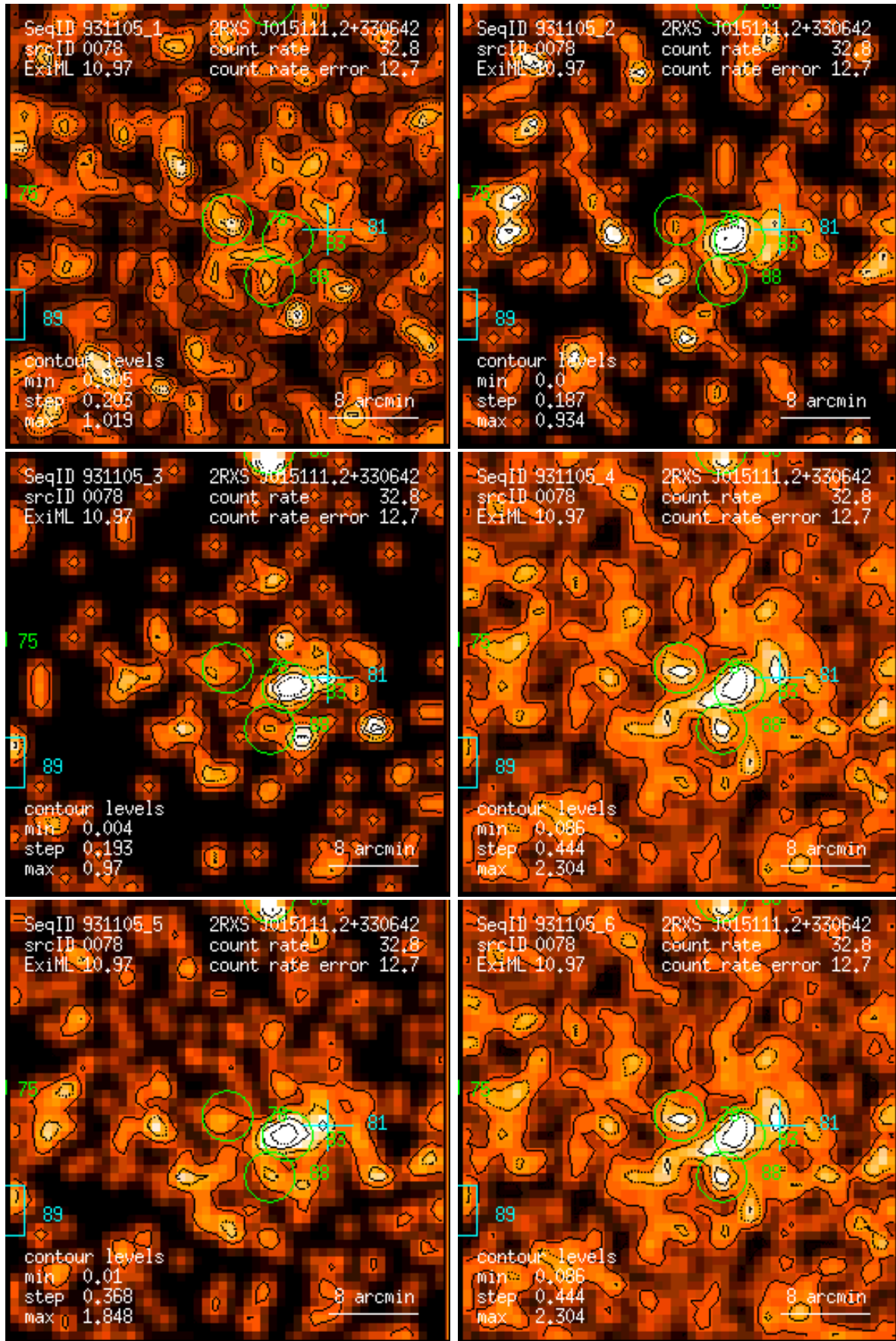
Figure 78: RASS 931105: detection 0078: band rate images, Gaussian filter: (1) PSPC channels 11 – 41, (2) 52 – 90, (3) 91 – 201, (4) 11 – 235, (5) 52 – 201, (6) 11 – 201. Broad band rates in counts/ks. Band rate contour levels in counts/ks/arcmin 2 .
