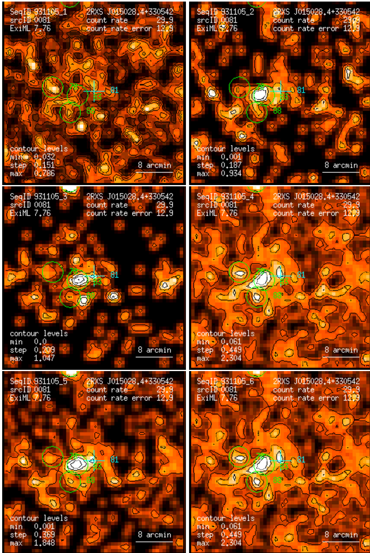
Figure 81: RASS 931105: detection 0081: band rate images, Gaussian filter: (1) PSPC channels 11 – 41, (2) 52 – 90, (3) 91 – 201, (4) 11 – 235, (5) 52 – 201, (6) 11 – 201. Broad band rates in counts/ks. Band rate contour levels in counts/ks/arcmin 2 .
