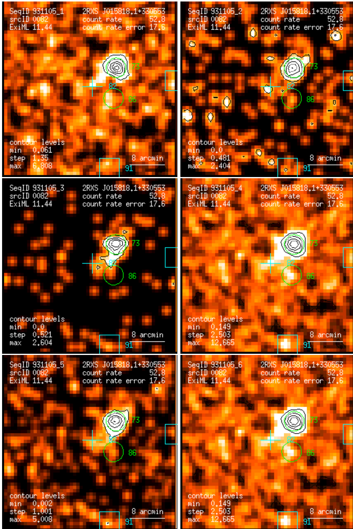
Figure 82: RASS 931105: detection 0082: band rate images, Gaussian filter: (1) PSPC channels 11 – 41, (2) 52 – 90, (3) 91 – 201, (4) 11 – 235, (5) 52 – 201, (6) 11 – 201. Broad band rates in counts/ks. Band rate contour levels in counts/ks/arcmin 2 .
