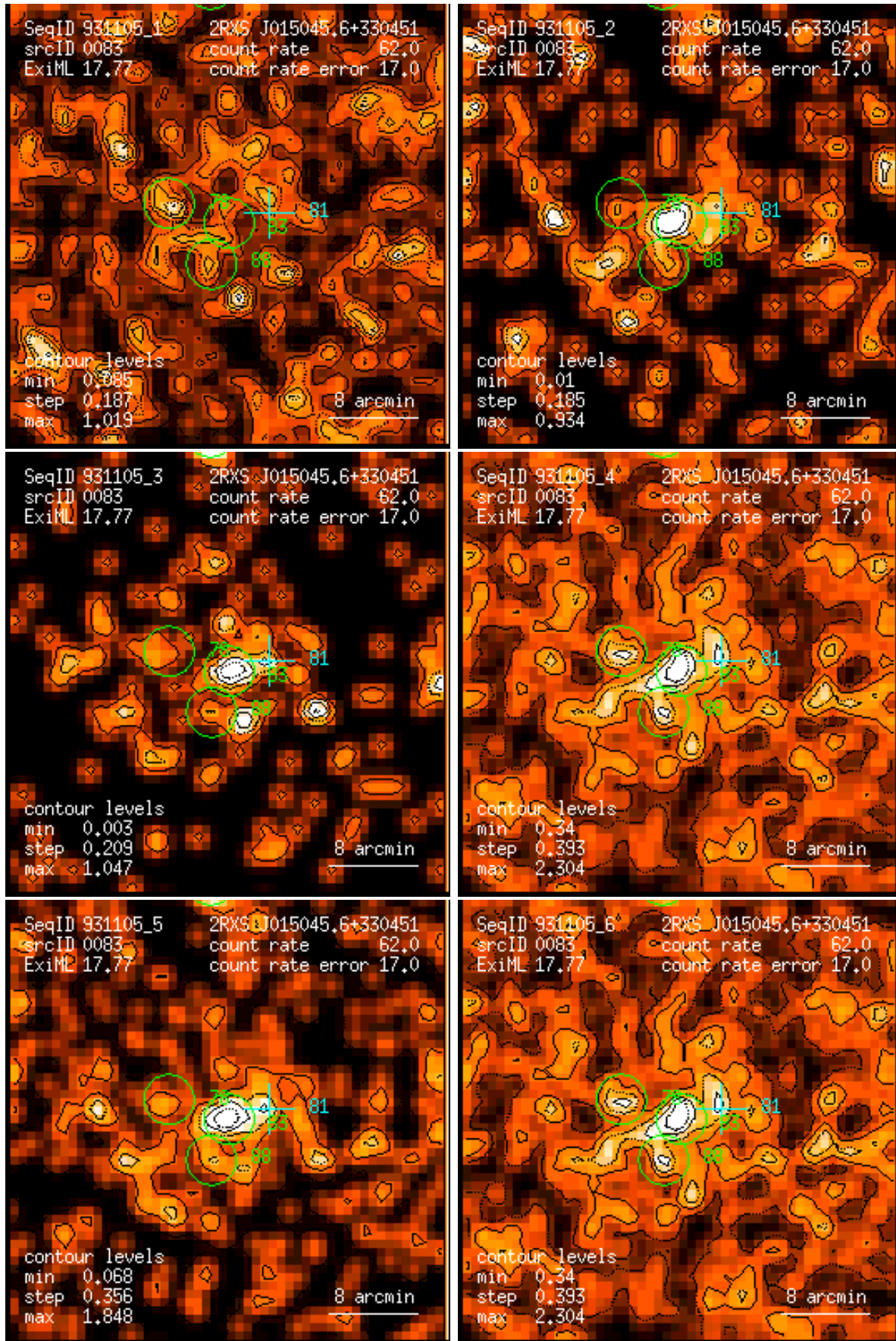
Figure 83: RASS 931105: detection 0083: band rate images, Gaussian filter: (1) PSPC channels 11 – 41, (2) 52 – 90, (3) 91 – 201, (4) 11 – 235, (5) 52 – 201, (6) 11 – 201. Broad band rates in counts/ks. Band rate contour levels in counts/ks/arcmin 2 .
