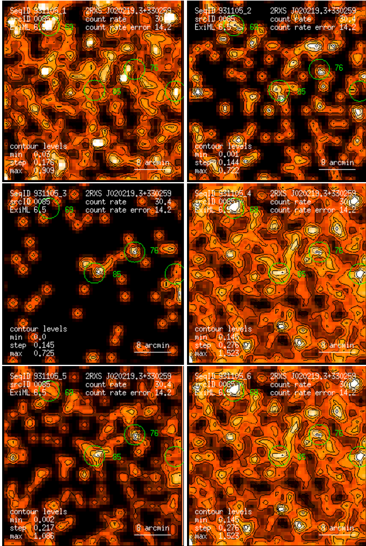
Figure 85: RASS 931105: detection 0085: band rate images, Gaussian filter: (1) PSPC channels 11 – 41, (2) 52 – 90, (3) 91 – 201, (4) 11 – 235, (5) 52 – 201, (6) 11 – 201. Broad band rates in counts/ks. Band rate contour levels in counts/ks/arcmin 2 .
