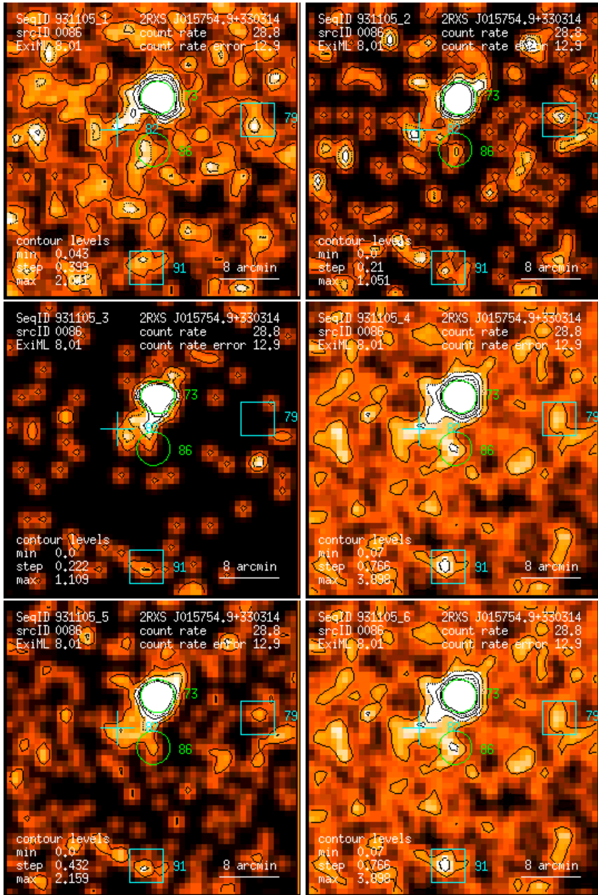
Figure 86: RASS 931105: detection 0086: band rate images, Gaussian filter: (1) PSPC channels 11 – 41, (2) 52 – 90, (3) 91 – 201, (4) 11 – 235, (5) 52 – 201, (6) 11 – 201. Broad band rates in counts/ks. Band rate contour levels in counts/ks/arcmin 2 .
