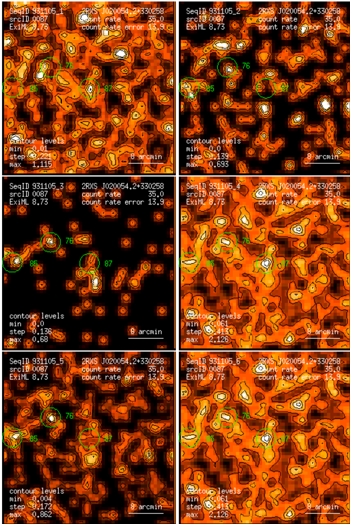
Figure 87: RASS 931105: detection 0087: band rate images, Gaussian filter: (1) PSPC channels 11 – 41, (2) 52 – 90, (3) 91 – 201, (4) 11 – 235, (5) 52 – 201, (6) 11 – 201. Broad band rates in counts/ks. Band rate contour levels in counts/ks/arcmin 2 .
