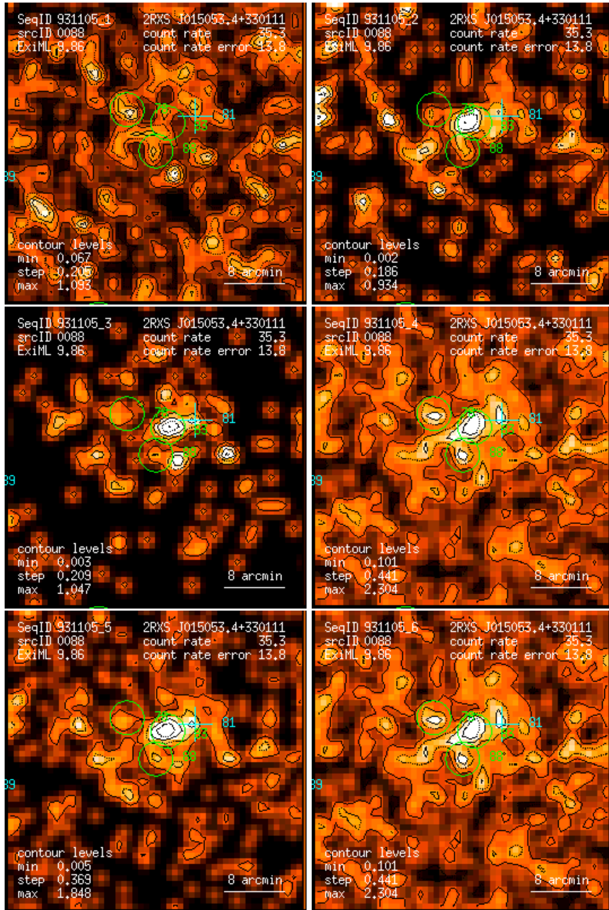
Figure 88: RASS 931105: detection 0088: band rate images, Gaussian filter: (1) PSPC channels 11 – 41, (2) 52 – 90, (3) 91 – 201, (4) 11 – 235, (5) 52 – 201, (6) 11 – 201. Broad band rates in counts/ks. Band rate contour levels in counts/ks/arcmin 2 .
