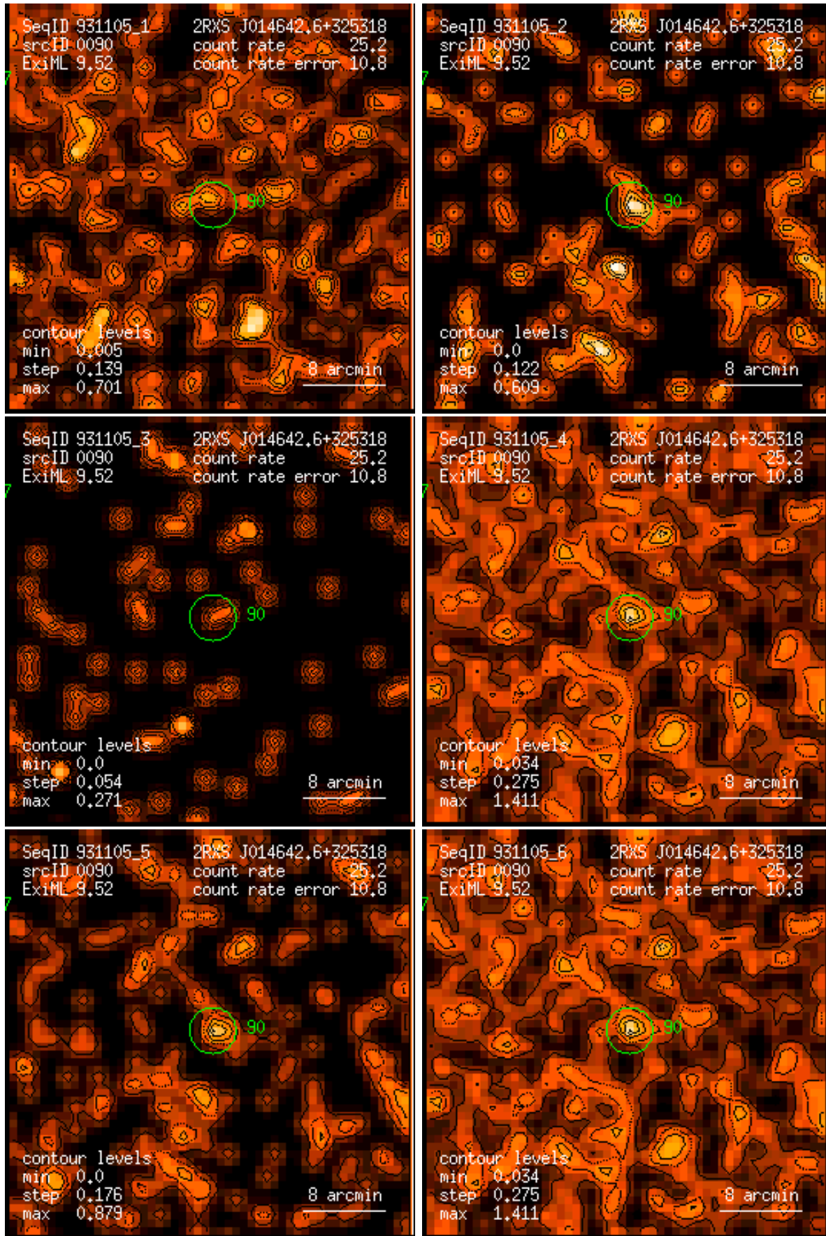
Figure 90: RASS 931105: detection 0090: band rate images, Gaussian filter: (1) PSPC channels 11 – 41, (2) 52 – 90, (3) 91 – 201, (4) 11 – 235, (5) 52 – 201, (6) 11 – 201. Broad band rates in counts/ks. Band rate contour levels in counts/ks/arcmin 2 .
