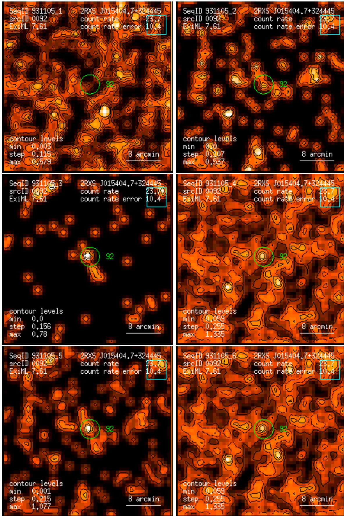
Figure 92: RASS 931105: detection 0092: band rate images, Gaussian filter: (1) PSPC channels 11 – 41, (2) 52 – 90, (3) 91 – 201, (4) 11 – 235, (5) 52 – 201, (6) 11 – 201. Broad band rates in counts/ks. Band rate contour levels in counts/ks/arcmin 2 .
