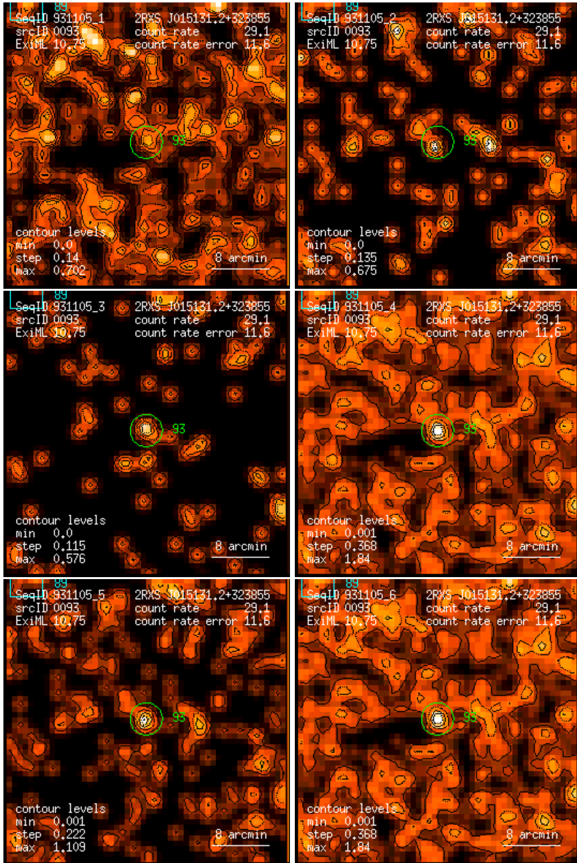
Figure 93: RASS 931105: detection 0093: band rate images, Gaussian filter: (1) PSPC channels 11 – 41, (2) 52 – 90, (3) 91 – 201, (4) 11 – 235, (5) 52 – 201, (6) 11 – 201. Broad band rates in counts/ks. Band rate contour levels in counts/ks/arcmin 2 .
