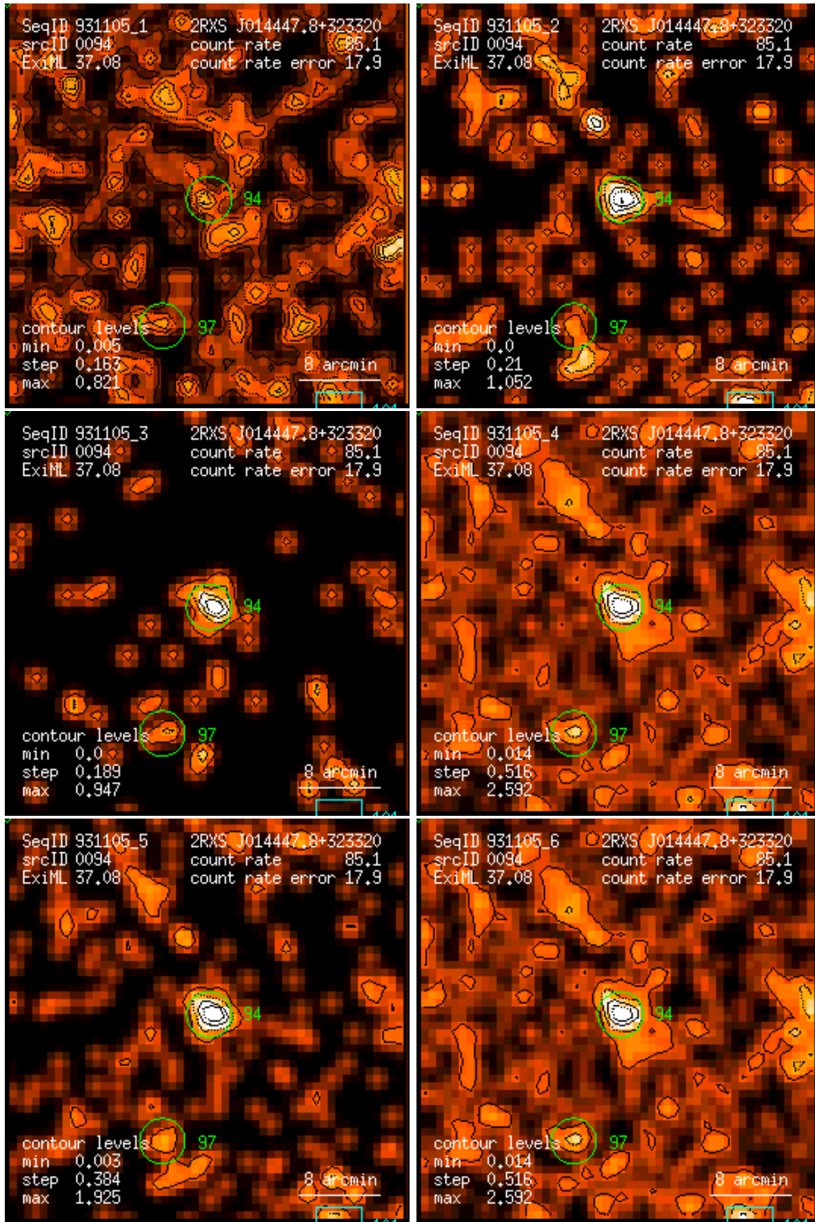
Figure 94: RASS 931105: detection 0094: band rate images, Gaussian filter: (1) PSPC channels 11 – 41, (2) 52 – 90, (3) 91 – 201, (4) 11 – 235, (5) 52 – 201, (6) 11 – 201. Broad band rates in counts/ks. Band rate contour levels in counts/ks/arcmin 2 .
