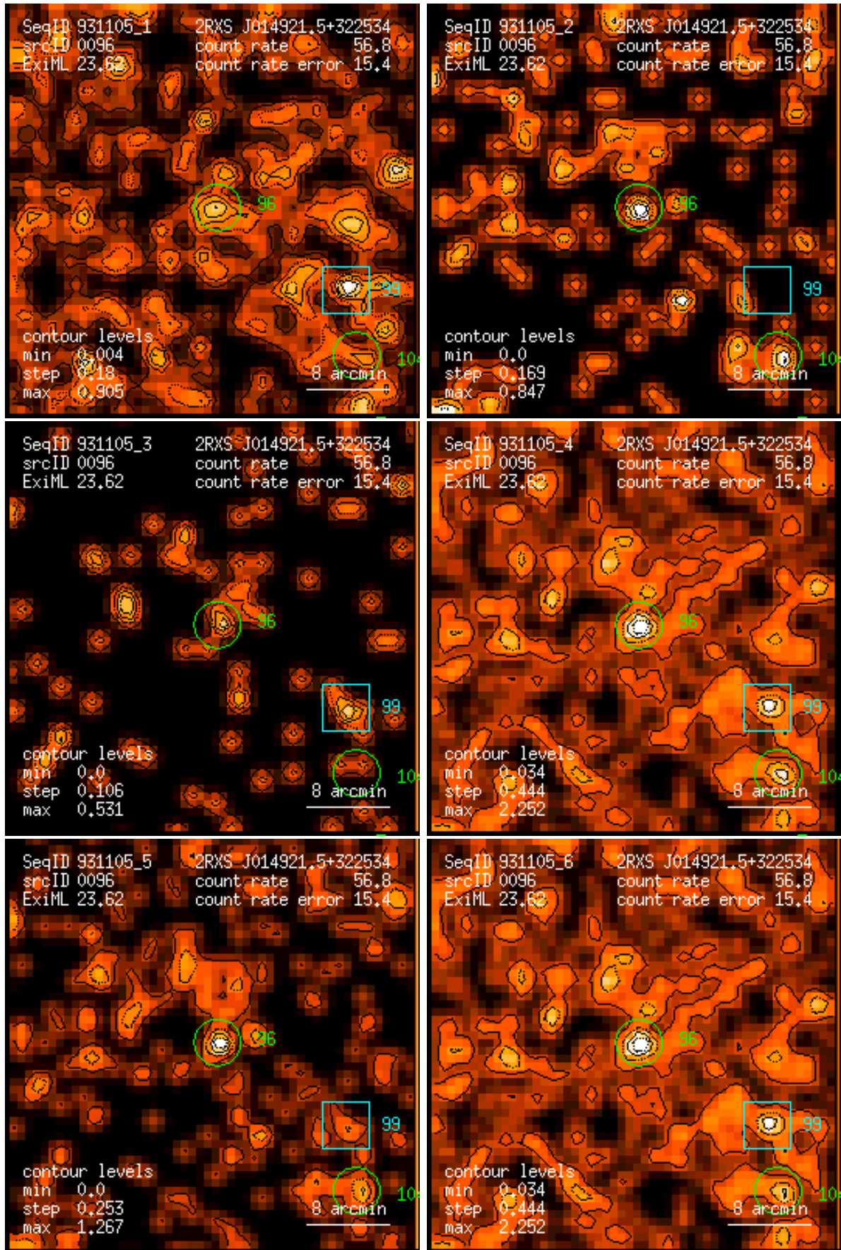
Figure 96: RASS 931105: detection 0096: band rate images, Gaussian filter: (1) PSPC channels 11 – 41, (2) 52 – 90, (3) 91 – 201, (4) 11 – 235, (5) 52 – 201, (6) 11 – 201. Broad band rates in counts/ks. Band rate contour levels in counts/ks/arcmin 2 .
