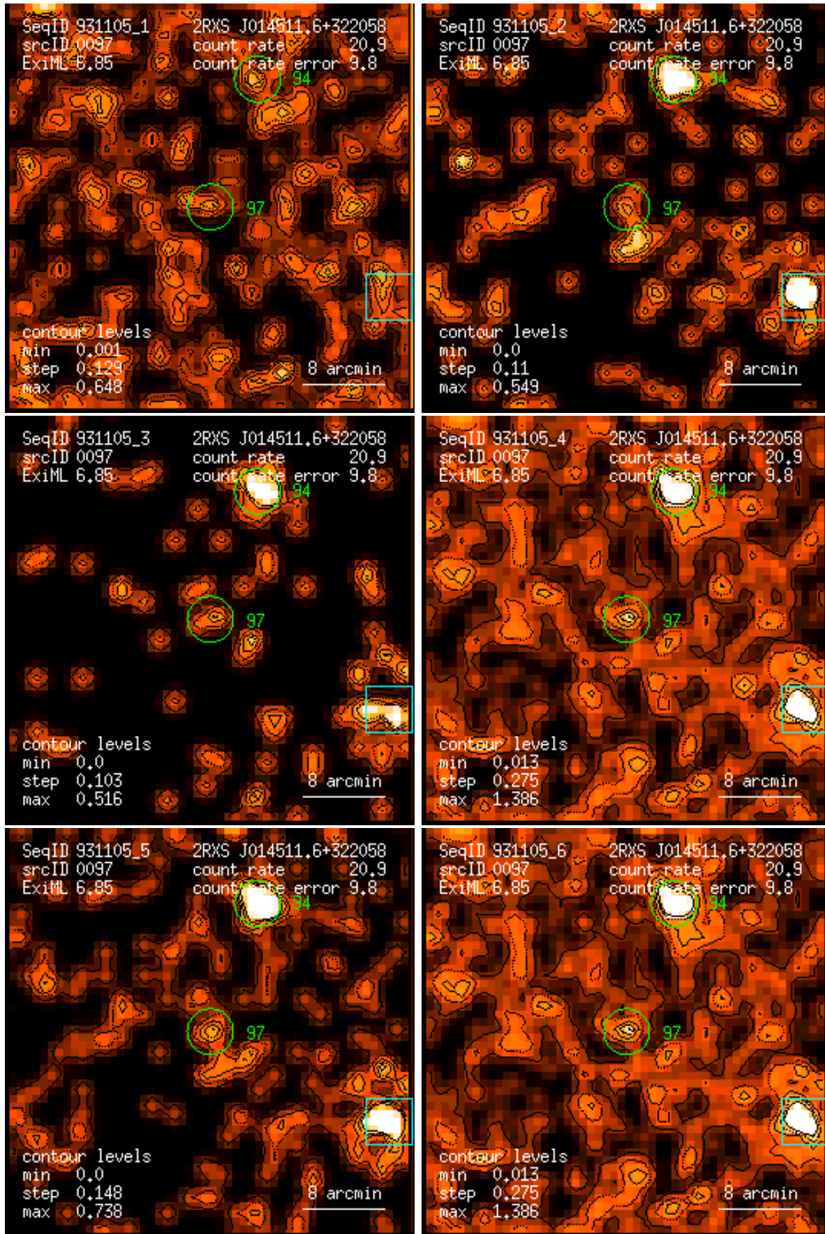
Figure 97: RASS 931105: detection 0097: band rate images, Gaussian filter: (1) PSPC channels 11 – 41, (2) 52 – 90, (3) 91 – 201, (4) 11 – 235, (5) 52 – 201, (6) 11 – 201. Broad band rates in counts/ks. Band rate contour levels in counts/ks/arcmin 2 .
