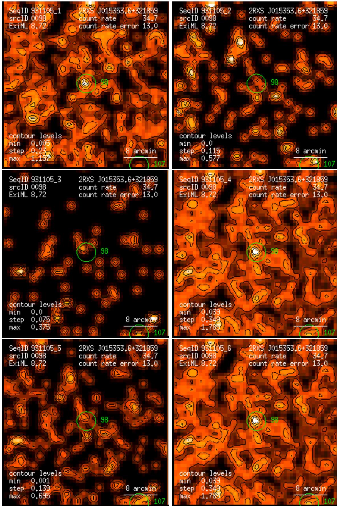
Figure 98: RASS 931105: detection 0098: band rate images, Gaussian filter: (1) PSPC channels 11 – 41, (2) 52 – 90, (3) 91 – 201, (4) 11 – 235, (5) 52 – 201, (6) 11 – 201. Broad band rates in counts/ks. Band rate contour levels in counts/ks/arcmin 2 .
