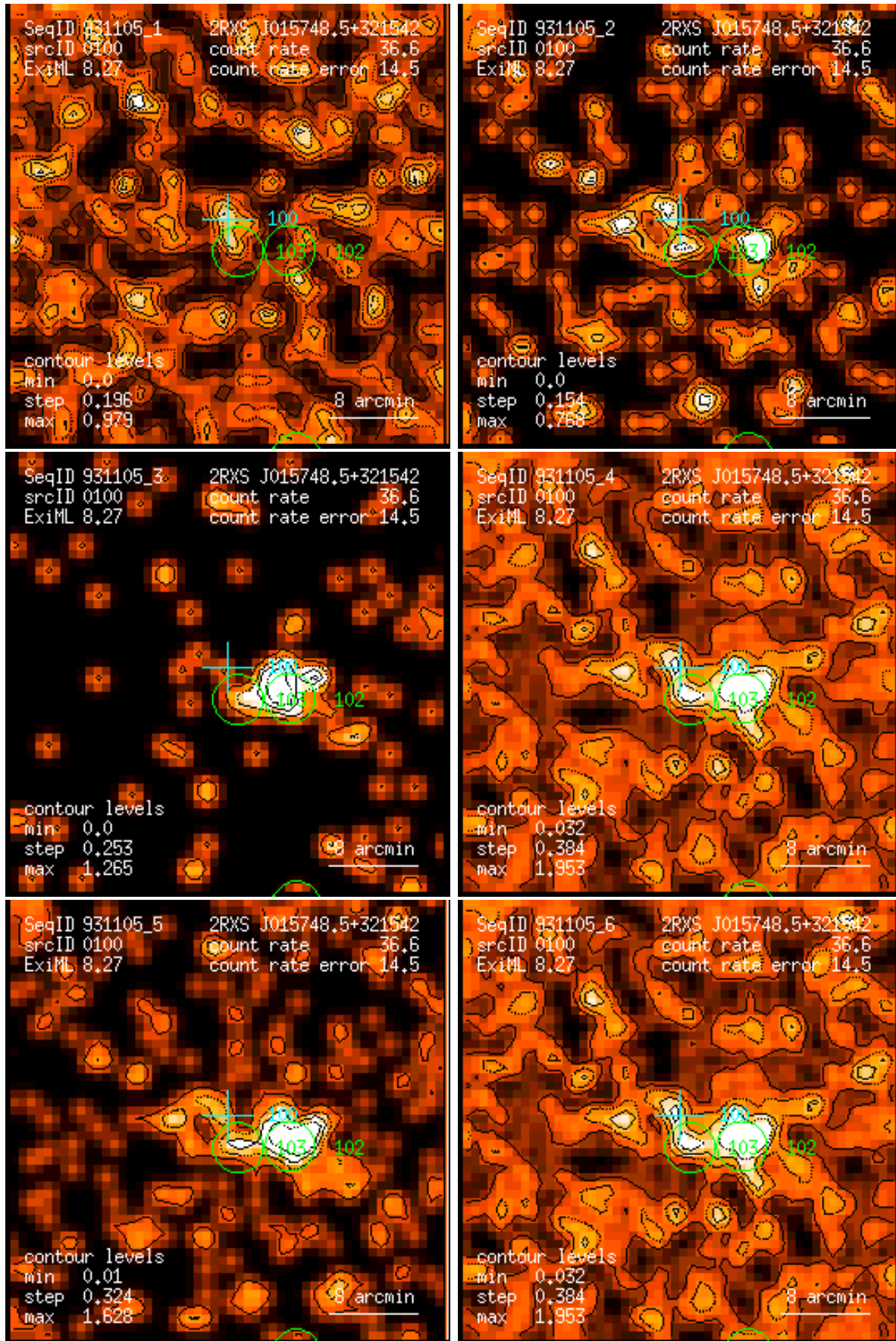
Figure 100: RASS 931105: detection 0100: band rate images, Gaussian filter: (1) PSPC channels 11 – 41, (2) 52 – 90, (3) 91 – 201, (4) 11 – 235, (5) 52 – 201, (6) 11 – 201. Broad band rates in counts/ks. Band rate contour levels in counts/ks/arcmin 2 .
