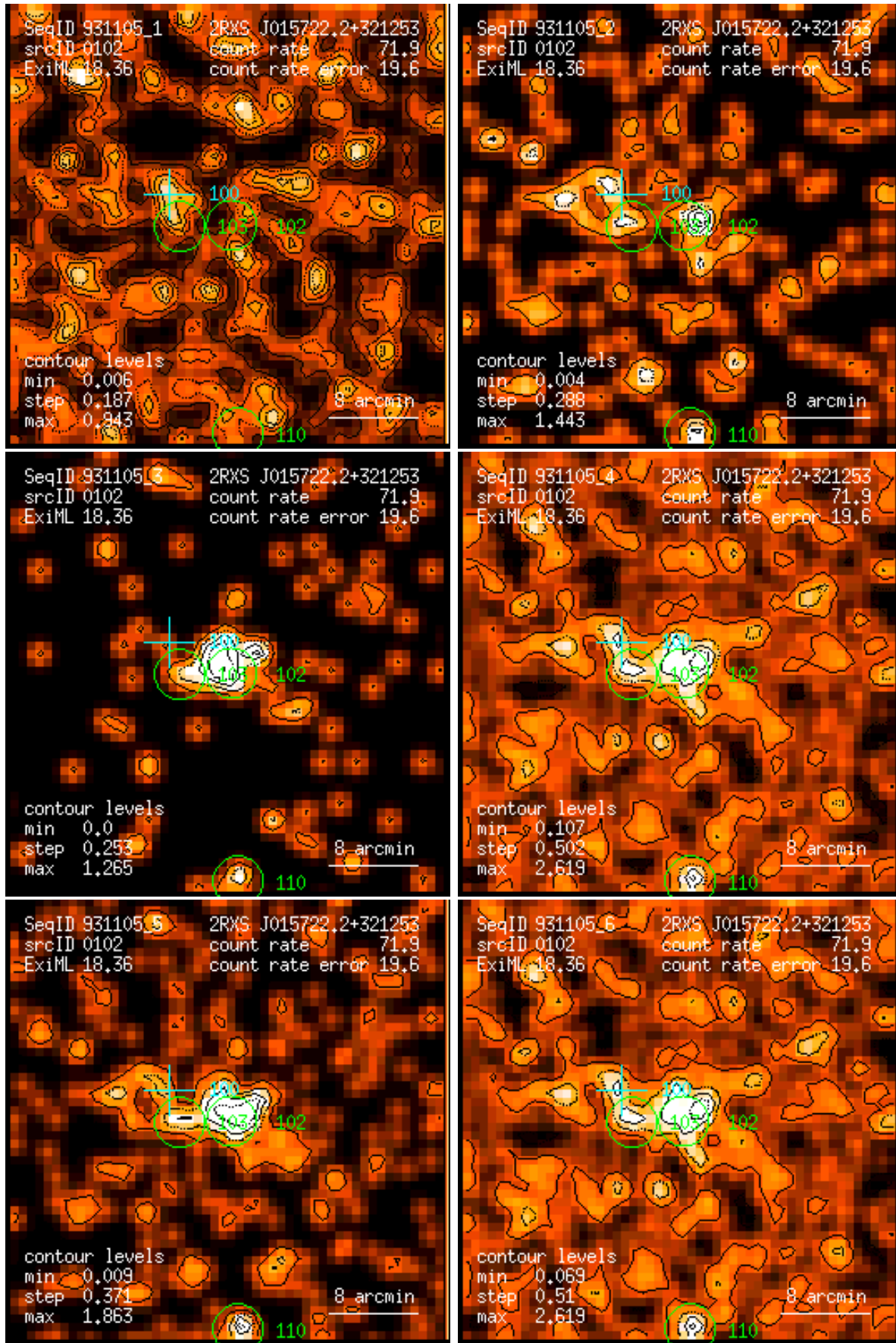
Figure 102: RASS 931105: detection 0102: band rate images, Gaussian filter: (1) PSPC channels 11 – 41, (2) 52 – 90, (3) 91 – 201, (4) 11 – 235, (5) 52 – 201, (6) 11 – 201. Broad band rates in counts/ks. Band rate contour levels in counts/ks/arcmin 2 .
